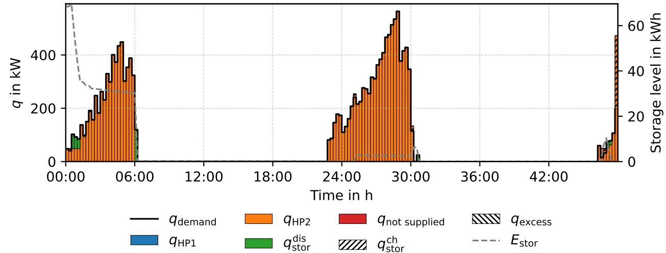
Heat balance - RP rp02 (CR)
