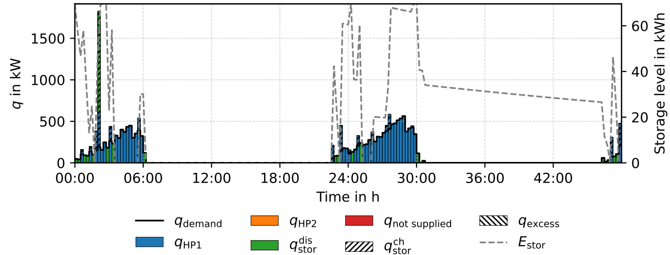
Heat balance - RP rp02 (LP)
