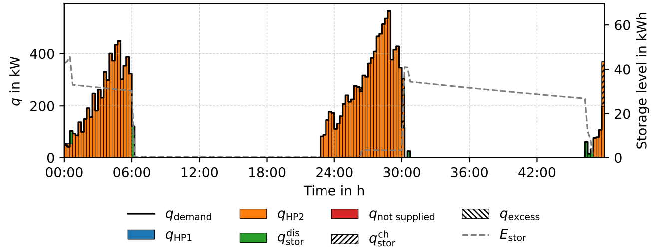
Heat balance - RP rp02 (PWL)
