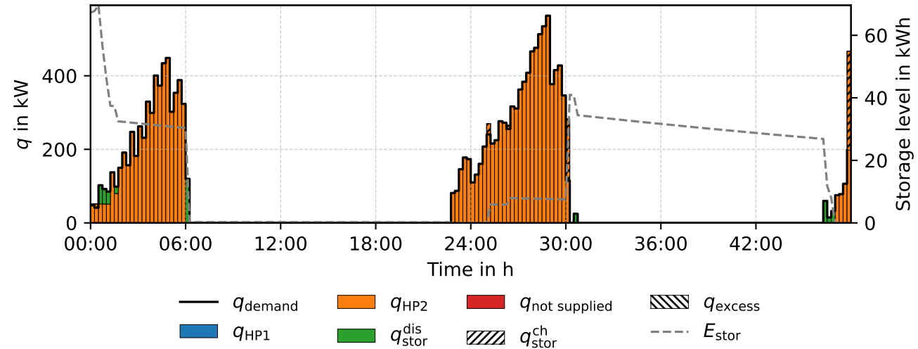
Heat balance - RP rp02 (PWLR)
