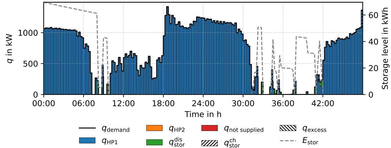
Heat balance - RP rp04 (LP)
