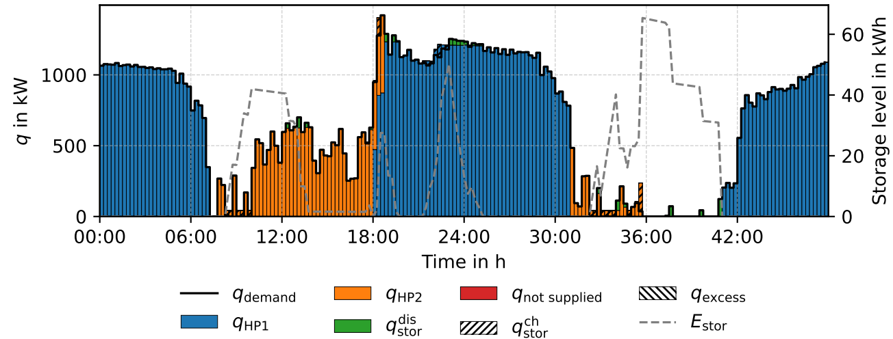
Heat balance - RP rp04 (PWL)
