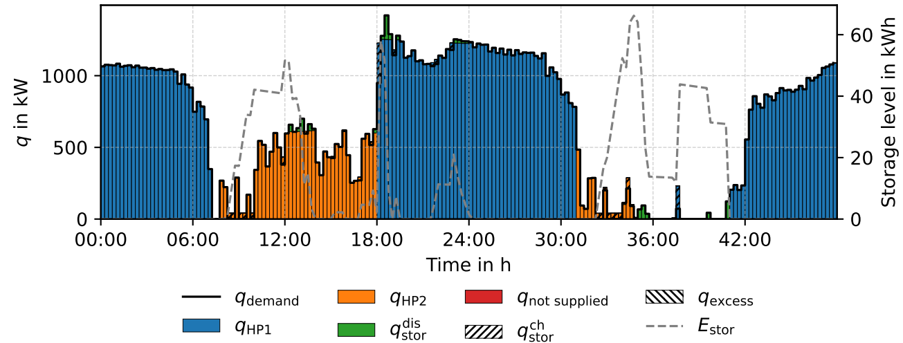
Heat balance - RP rp04 (PWLR)
