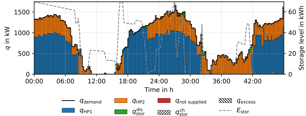
Heat balance – RP rp05 (CR)
