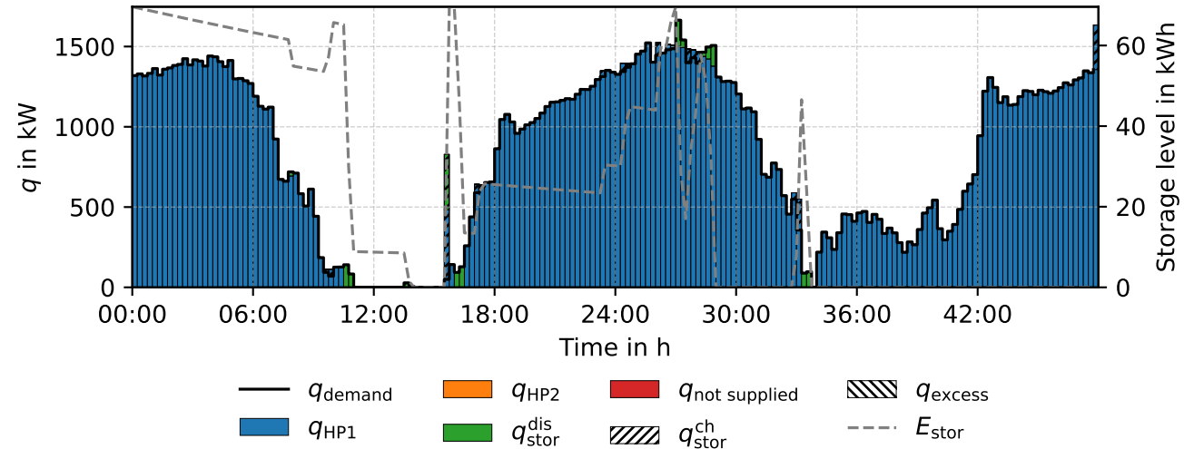
Heat balance - RP rp05 (LP)
