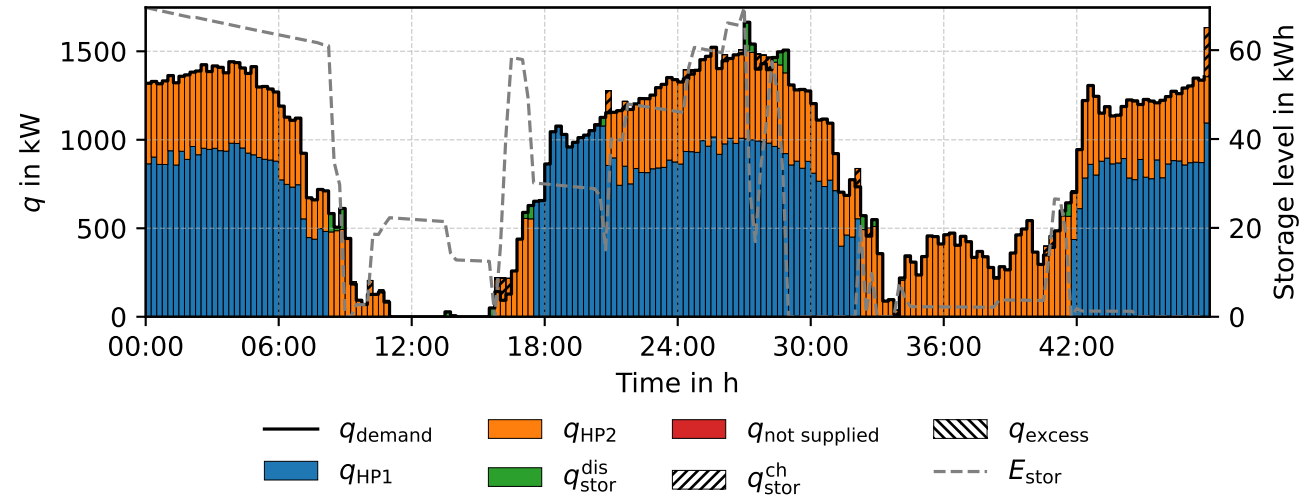
Heat balance - RP rp05 (PWL)
