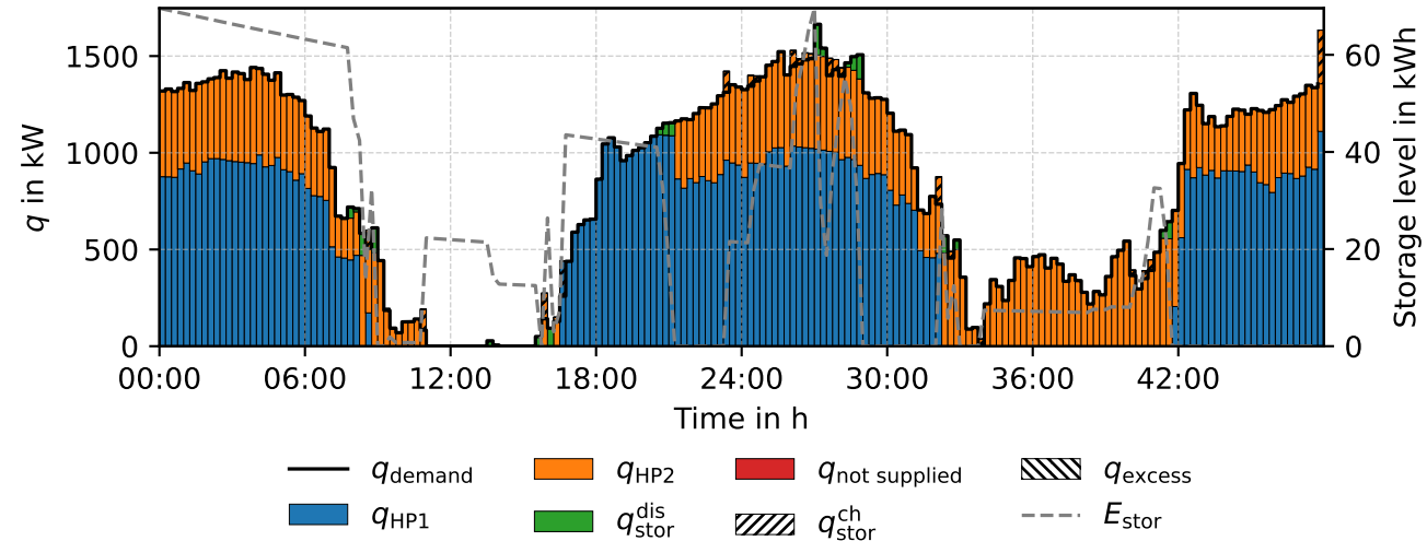
Heat balance – RP rp05 (PWLR)
