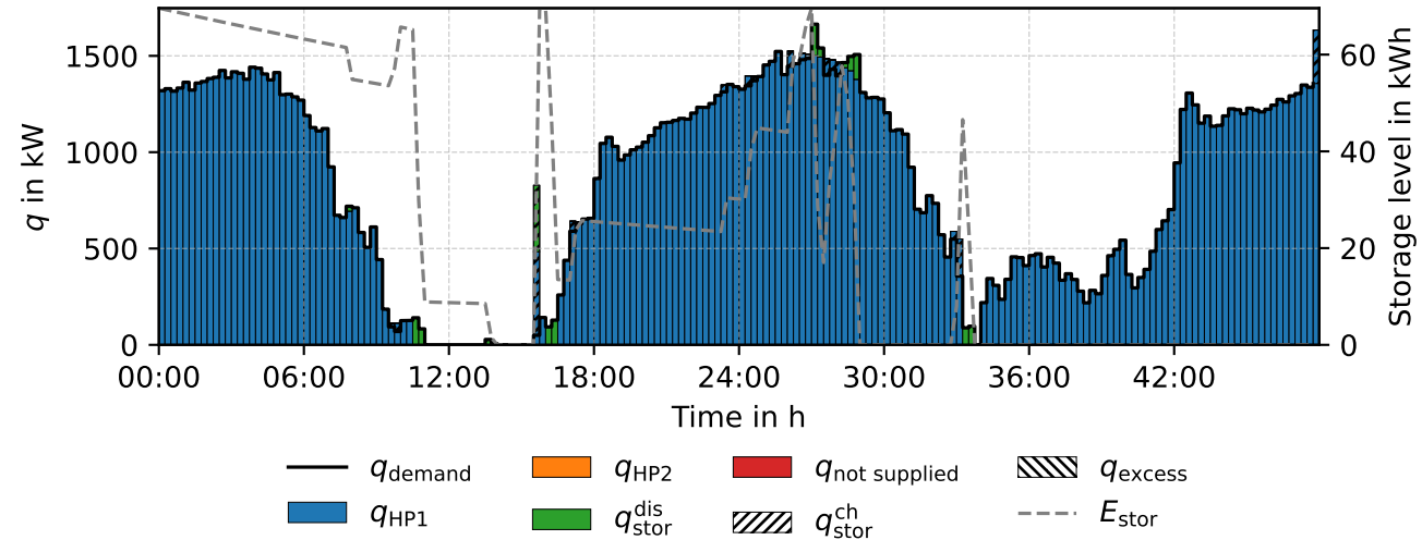
Heat balance - RP rp05 (UC)
