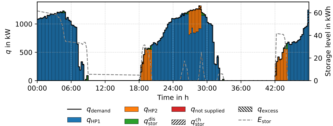
Heat balance – RP rp06 (CR)
