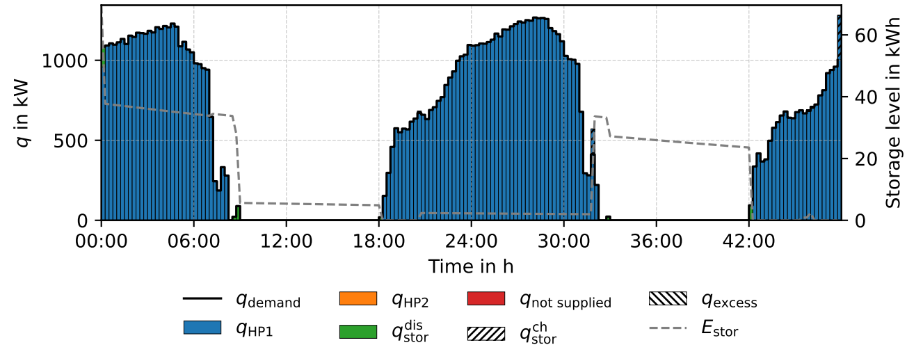
Heat balance - RP rp06 (LP)
