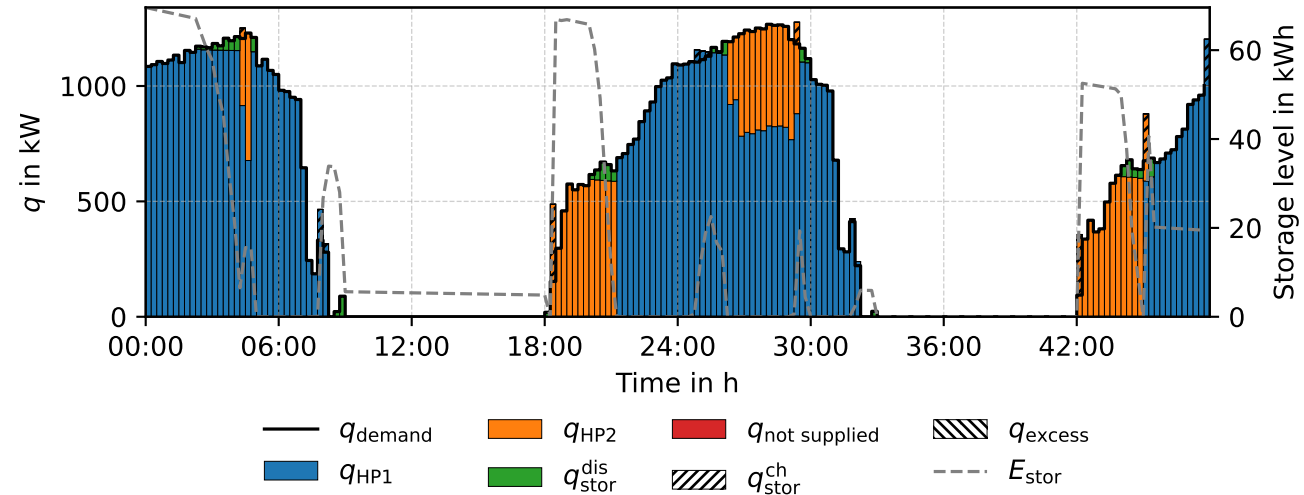
Heat balance - RP rp06 (PWL)
