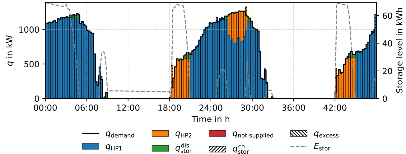
Heat balance - RP rp06 (PWLR)
