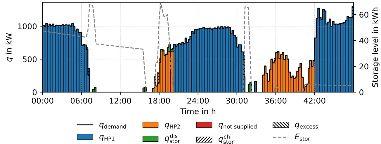
Heat balance – RP rp08 (CR)
