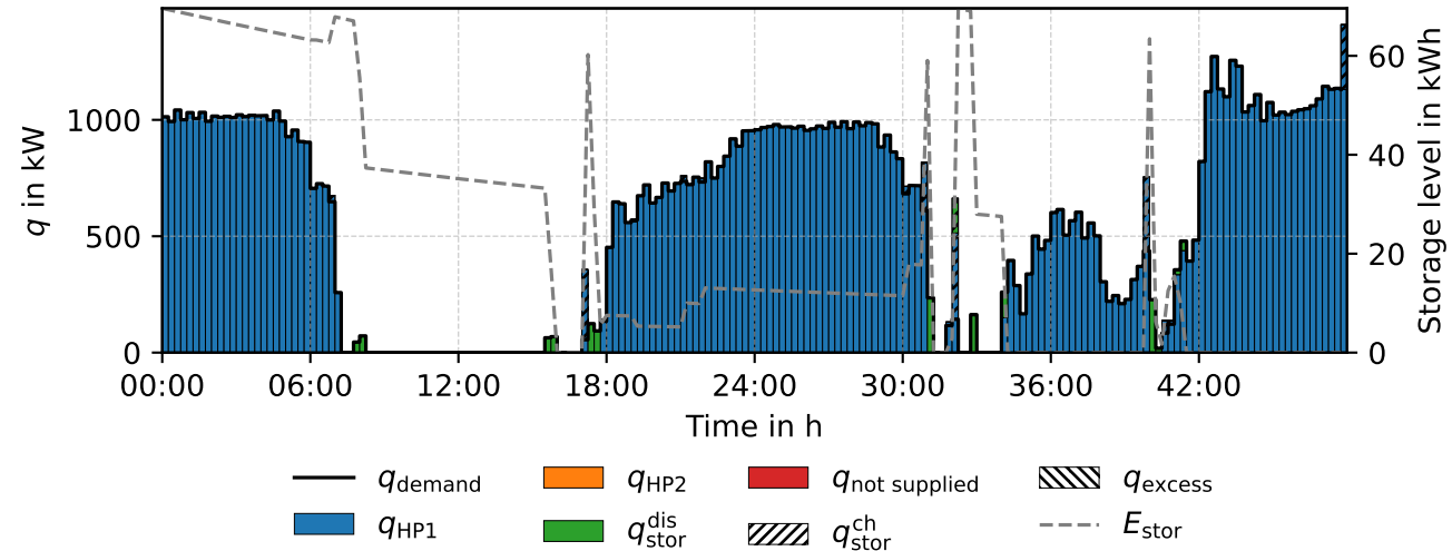
Heat balance - RP rp08 (LP)
