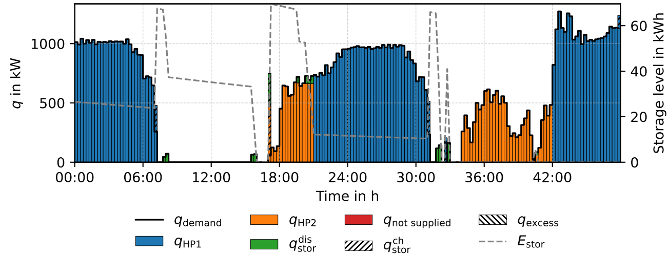
Heat balance - RP rp08 (PWL)
