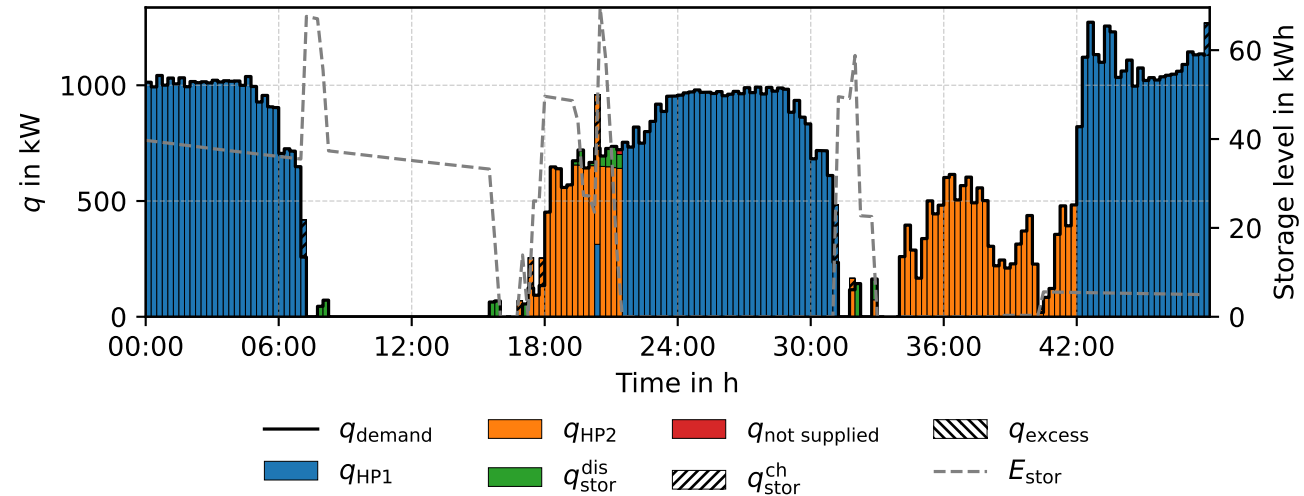
Heat balance - RP rp08 (PWLR)
