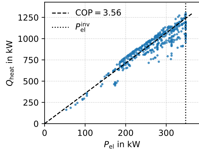
Heat Pump Performance Map (CR)
