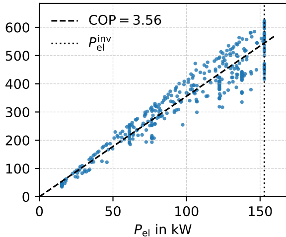
Heat Pump Performance Map (CR)
