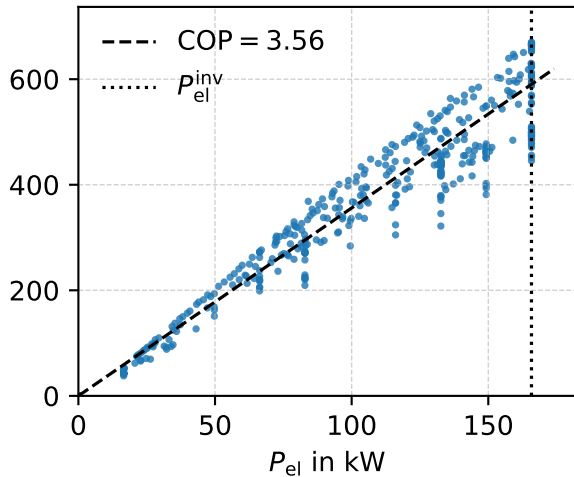
Heat Pump Performance Map (PWL)
