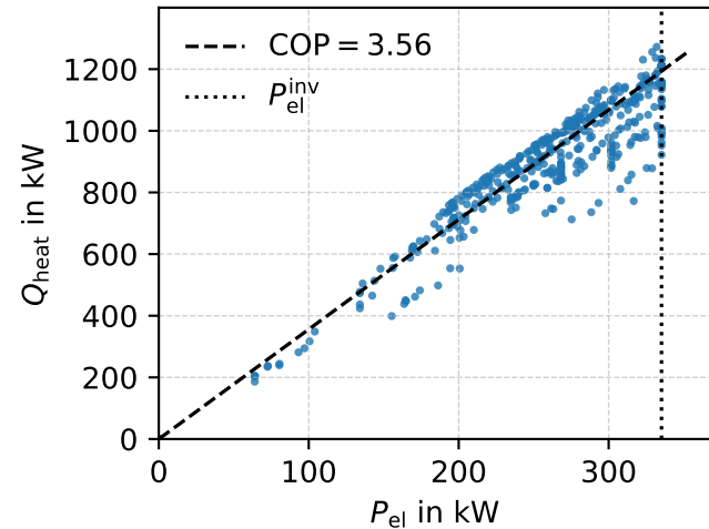
Heat Pump Performance Map (PWL)
