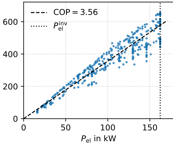
Heat Pump Performance Map (PWLR)
