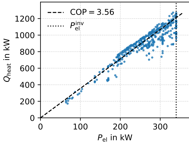
Heat Pump Performance Map (PWLR)
