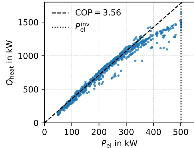
Heat Pump Performance Map (UC)
