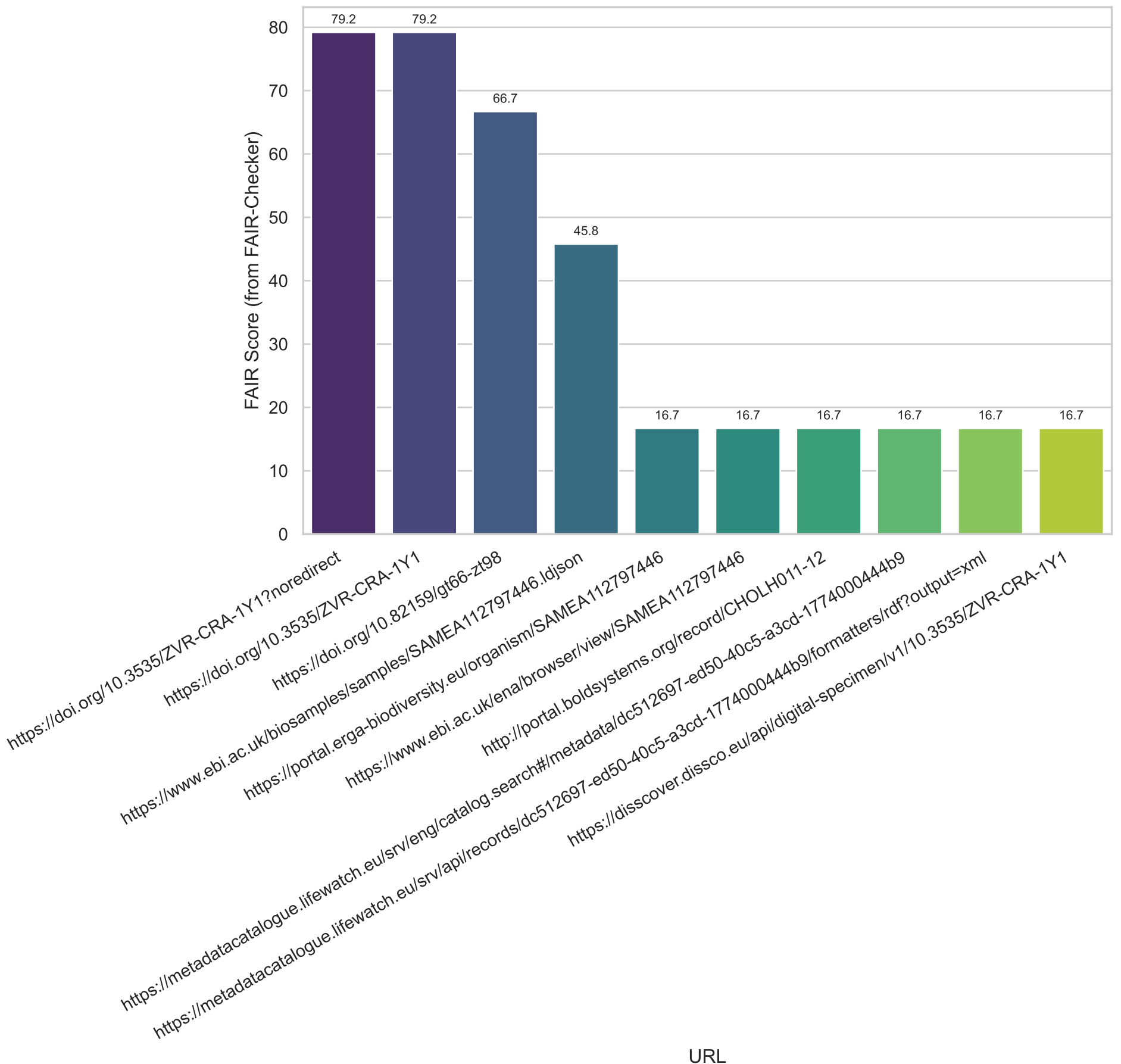
Example biodiversity resources FAIR scores 2026-04-13
