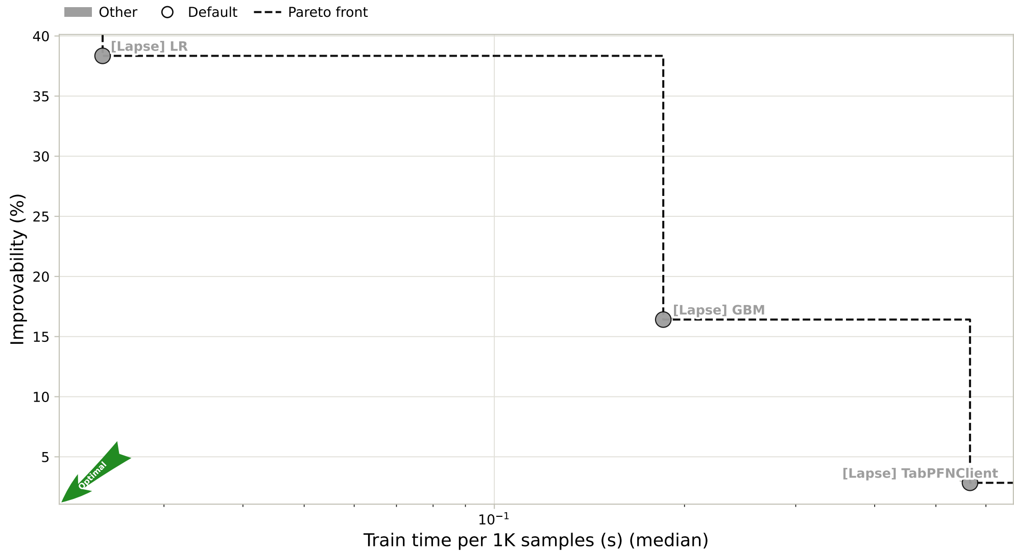
Improvability vs Train Time
