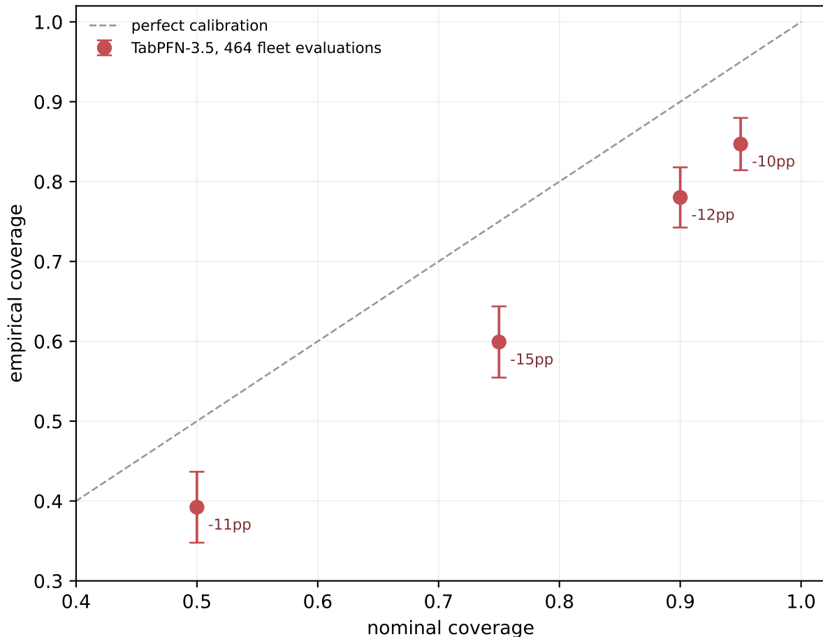
Do the intervals contain the truth as often as they claim? 464 fleet evaluations, held-out diagonals, 95% binomial bars
