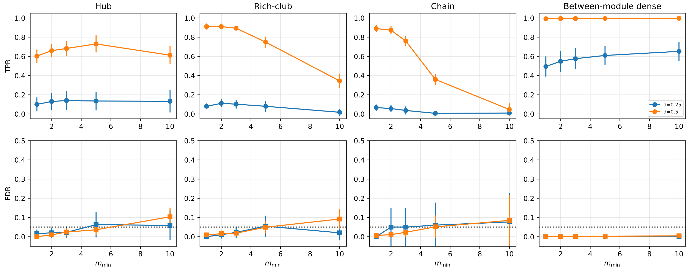
FBC-TFNBS: Sensitivity to m_{\min}
