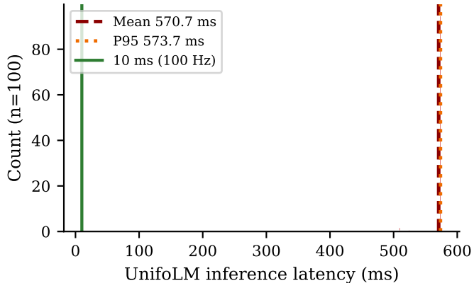
(a) Live UnifoLM-VLA-Base (G1_Clean_Table)
