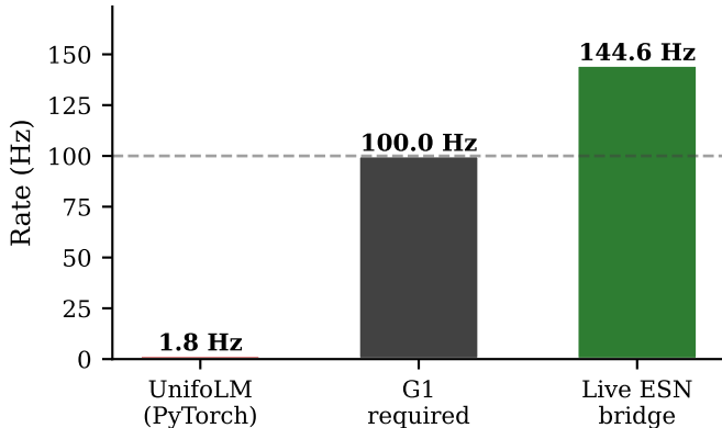
(b) Frequency gap \approx 57\times vs 100 Hz
