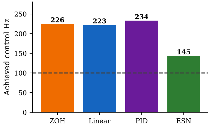
(b) Achieved rate (10 s live UnifoLM)
