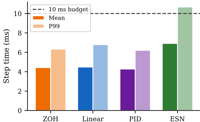
(a) Live dual-process step latency
