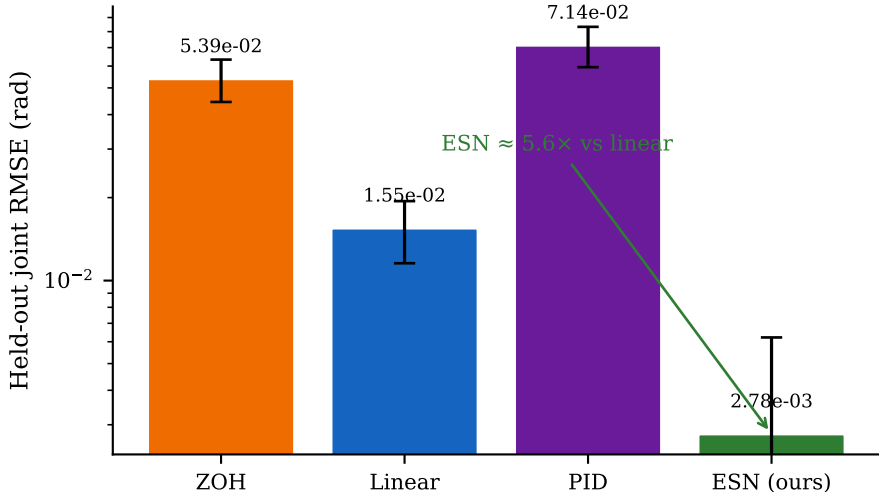
Open-loop upsample RMSE (40 held-out wipe eps)
