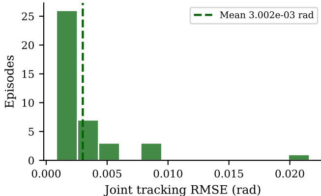
(a) Dataset-oracle ESN RMSE (n=40)
