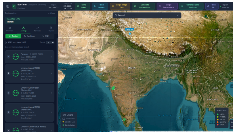
Figure 6.7: Live ranked-analog panel for Tso Morari, captured independently from the running application: Pangong returned as rank 1 at 98.9% displayed similarity, confirming Table 6.11.
