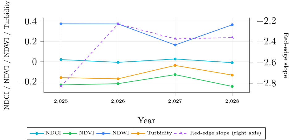
Figure 6.4: Beas (Maharana Pratap Sagar) — projected index trajectory, 2025–2028 (dashed vertical line marks the anchor year; Red-edge slope on the right axis).
