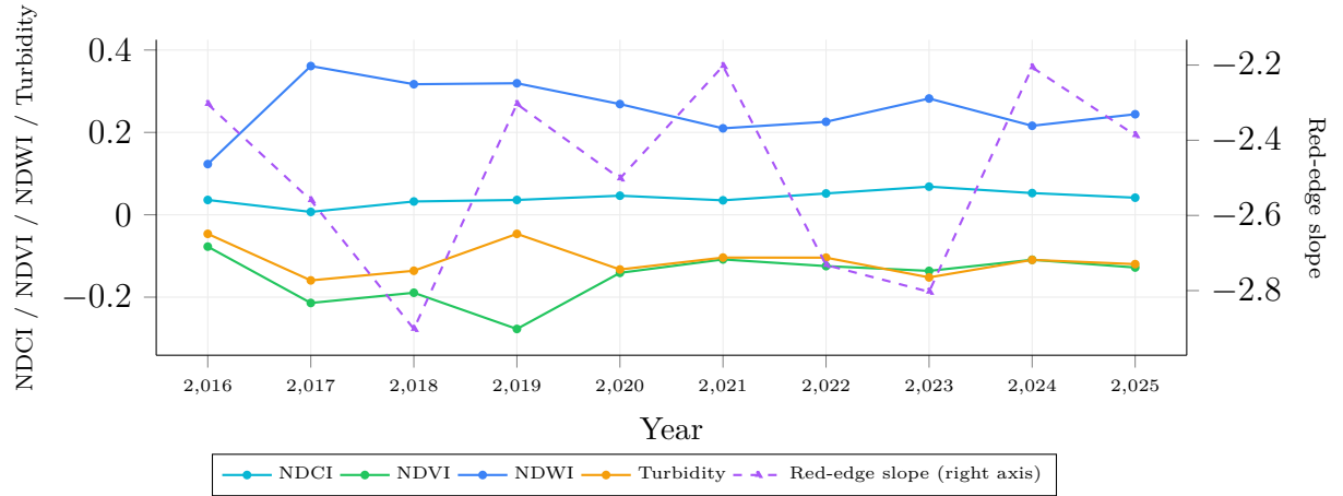
Figure 6.1: Chilika — measured index trajectory, 2016–2025 (10 years; NDCI/NDVI/NDWI/Turbidity on the left axis, Red-edge slope on the right).
