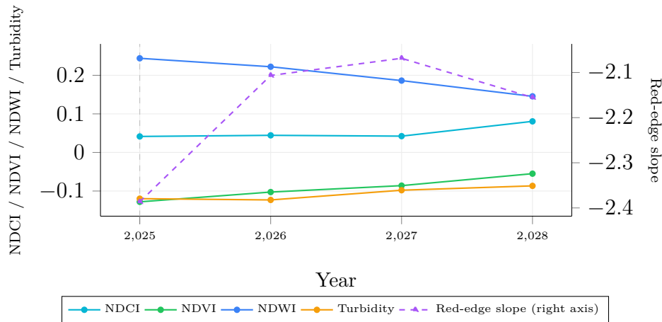
Figure 6.2: Chilika — projected index trajectory, 2025–2028 (dashed vertical line marks the anchor year; Red-edge slope on the right axis).
