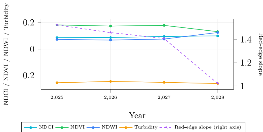
Figure 6.12: Sasthamcotta — projected index trajectory, 2025–2028 (dashed vertical line marks the anchor year; Red-edge slope on the right axis).
