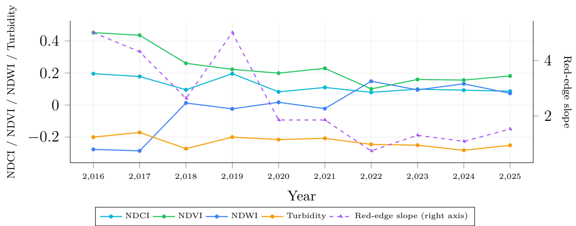
Figure 6.11: Sasthamcotta — measured index trajectory, 2016–2025 (10 years; NDCI/NDVI/NDWI/Turbidity on the left axis, Red-edge slope on the right).
