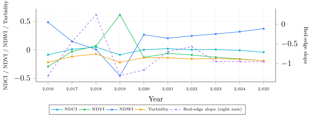
Figure 6.5: Tawa Reservoir — measured index trajectory, 2016–2025 (10 years; NDCI/NDVI/NDWI/Turbidity on the left axis, Red-edge slope on the right).
