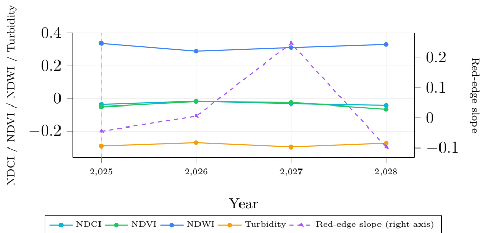
Figure 6.9: Tso Morari — projected index trajectory, 2025–2028 (dashed vertical line marks the anchor year; Red-edge slope on the right axis).
