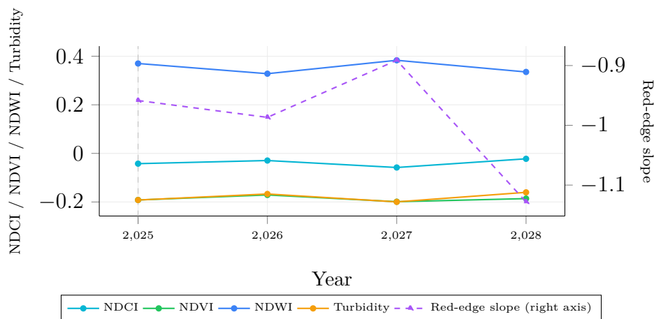
Figure 6.6: Tawa Reservoir — projected index trajectory, 2025–2028 (dashed vertical line marks the anchor year; Red-edge slope on the right axis).
