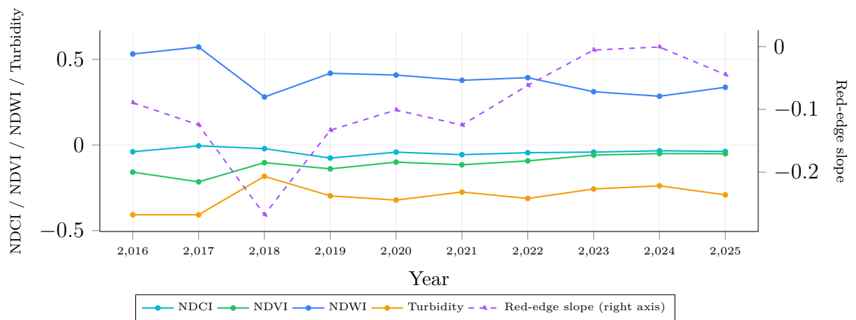
Figure 6.8: Tso Morari — measured index trajectory, 2016–2025 (10 years; NDCI/NDVI/NDWI/Turbidity on the left axis, Red-edge slope on the right).
