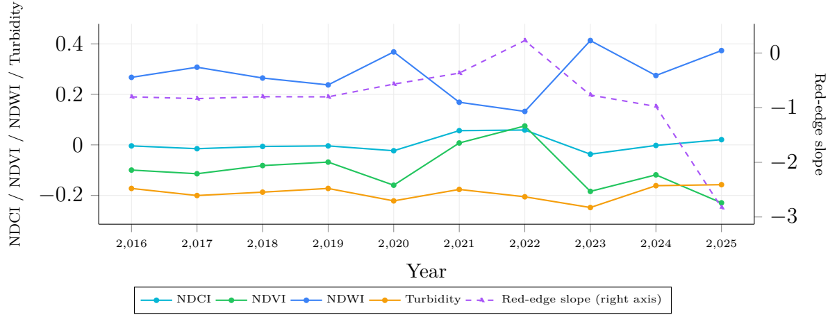
Figure 6.3: Beas (Maharana Pratap Sagar) — measured index trajectory, 2016–2025 (10 years; NDCI/NDVI/NDWI/Turbidity on the left axis, Red-edge slope on the right).
