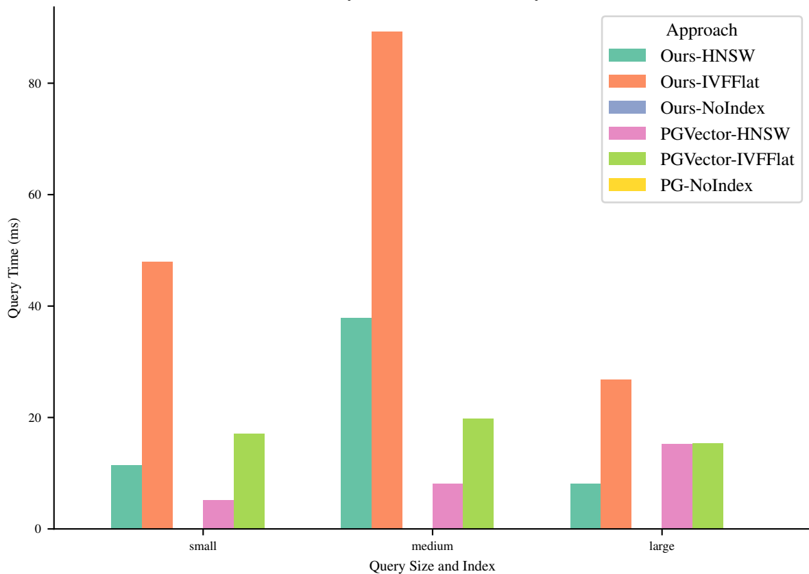
Query Time (ms) for Query 5
