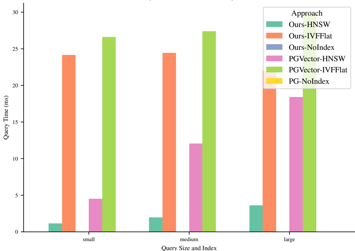
Query Time (ms) for Query 11
