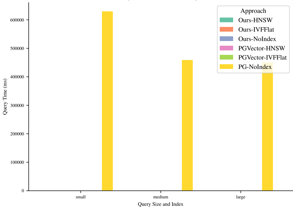
Query Time (ms) for Query 12
