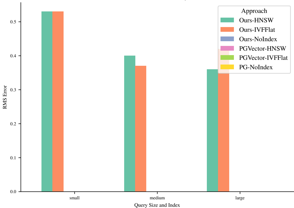
RMS Error for Query 8
