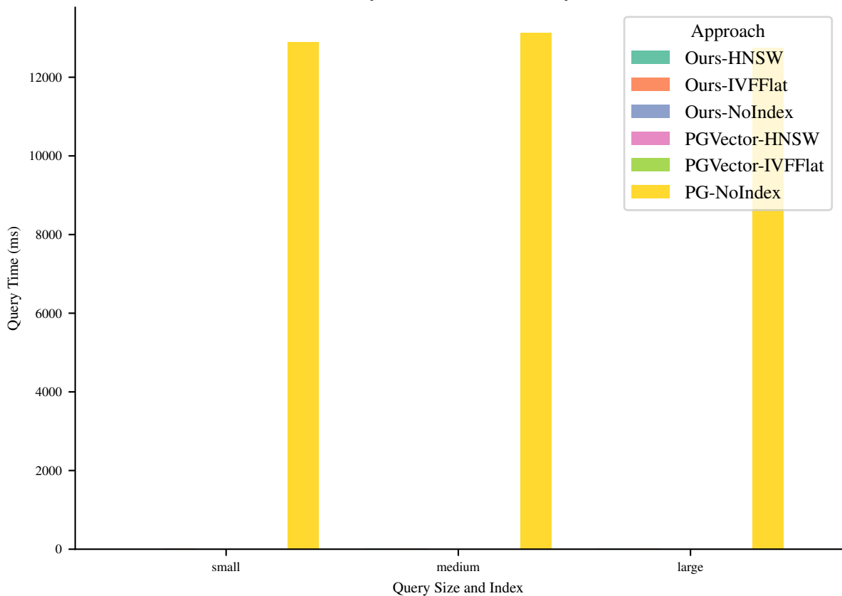
Query Time (ms) for Query 8
