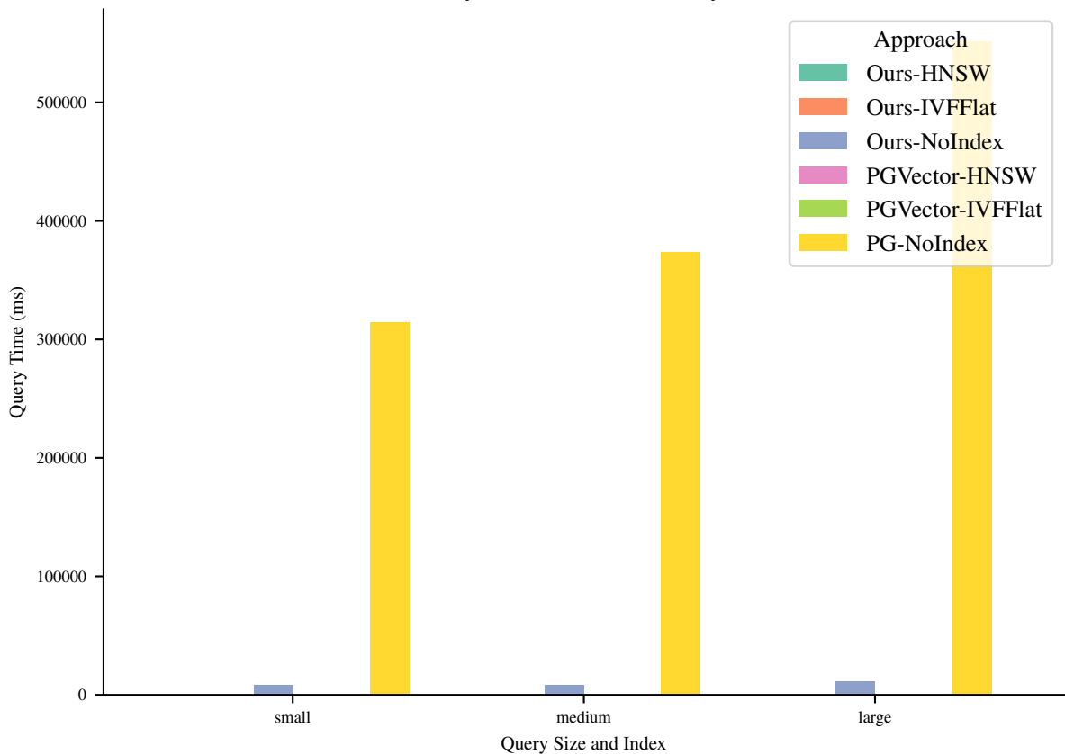
Query Time (ms) for Query 34
