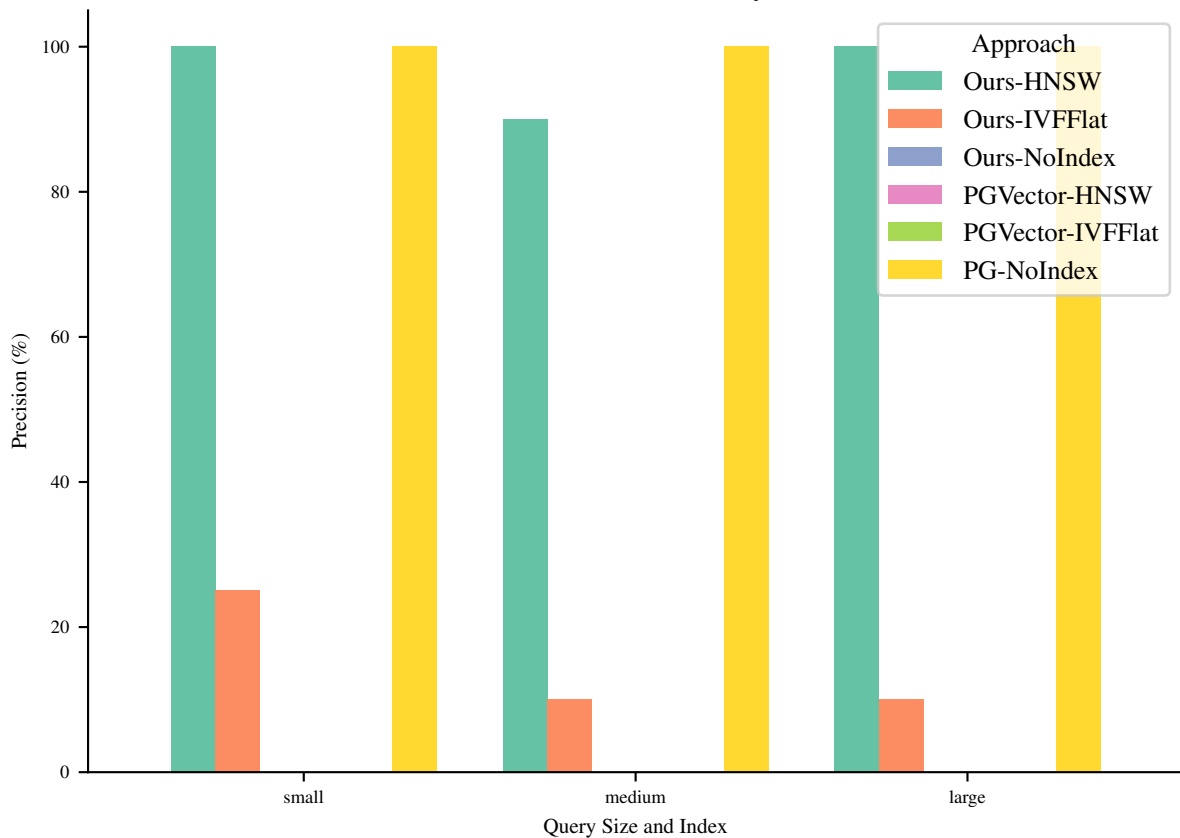
Precision (%) for Query 30
