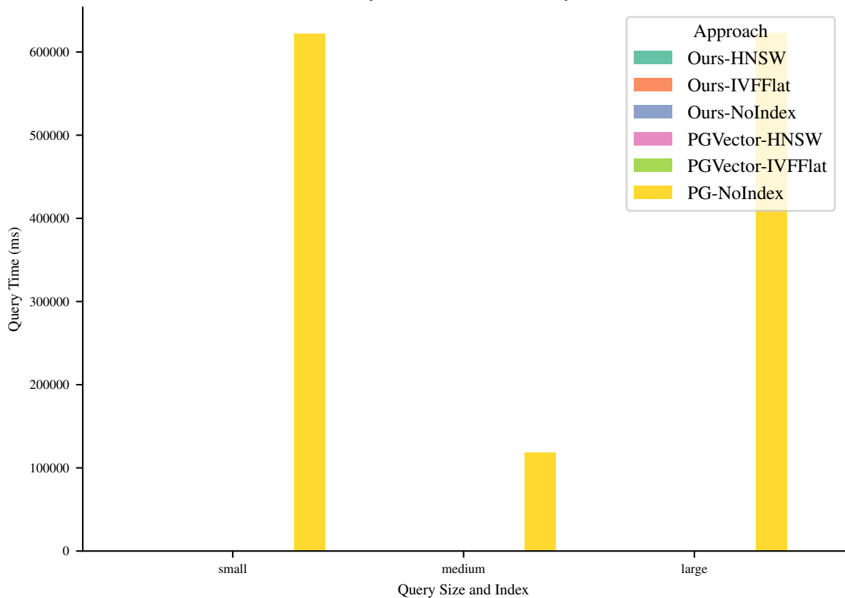
Query Time (ms) for Query 31
