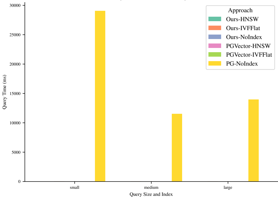
Query Time (ms) for Query 29
