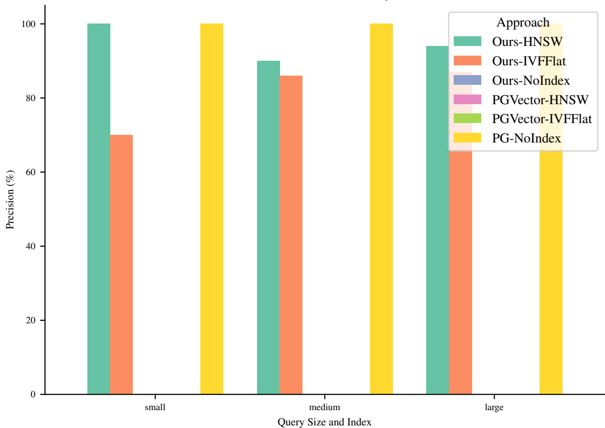
Precision (%) for Query 39
