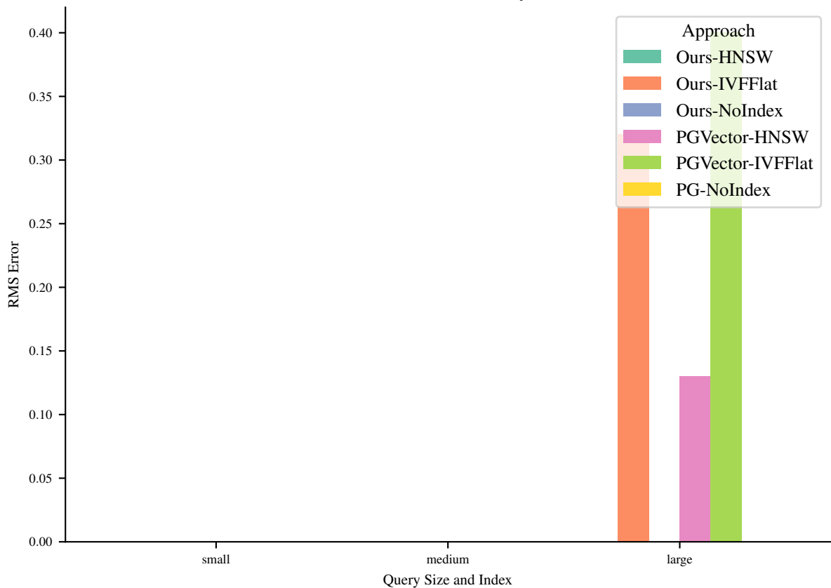
RMS Error for Query 11
