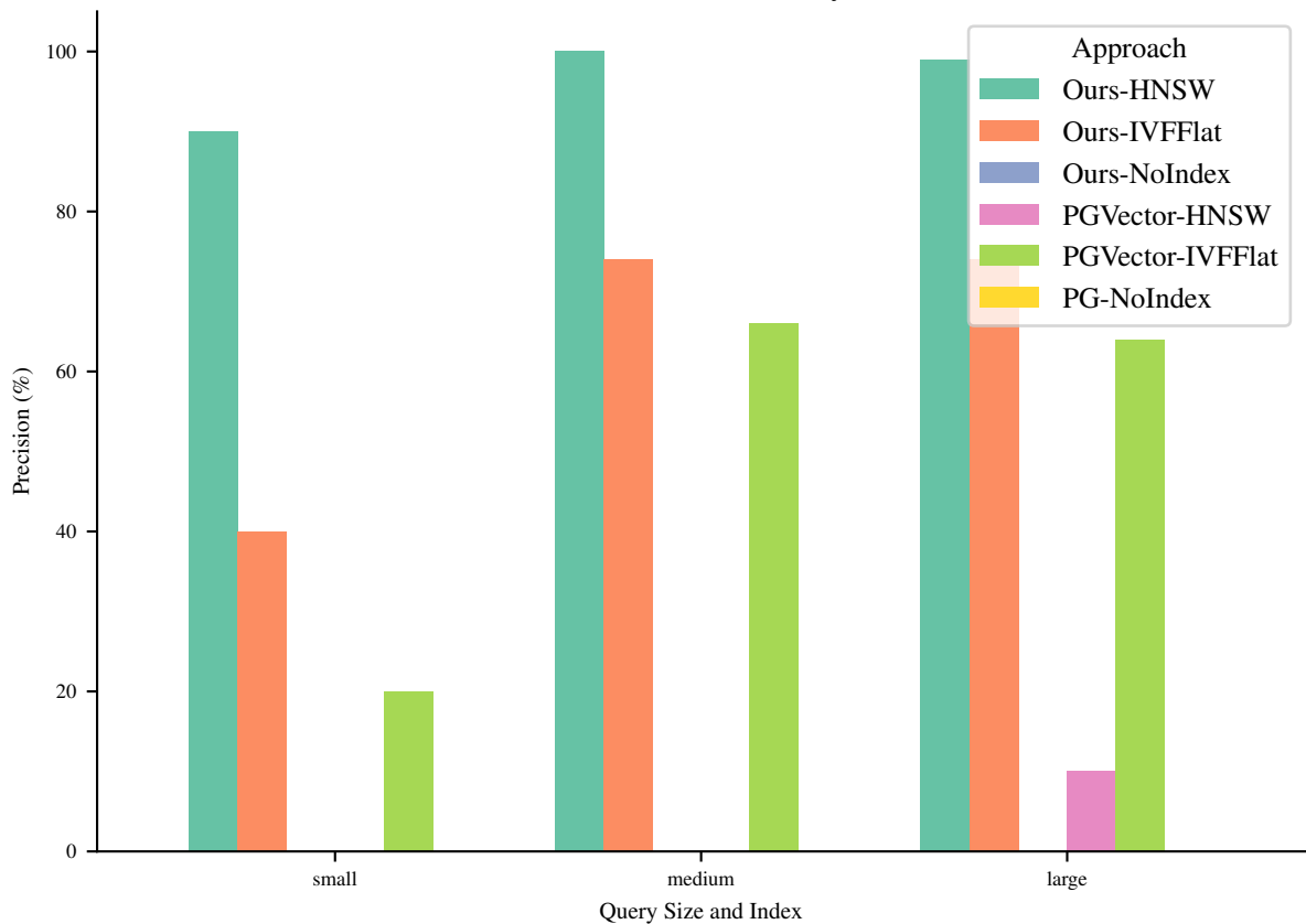
Precision (%) for Query 20
