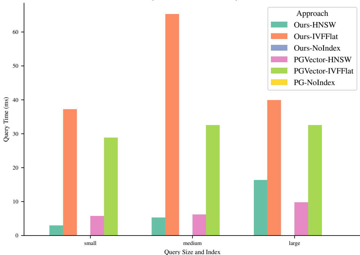
Query Time (ms) for Query 38
