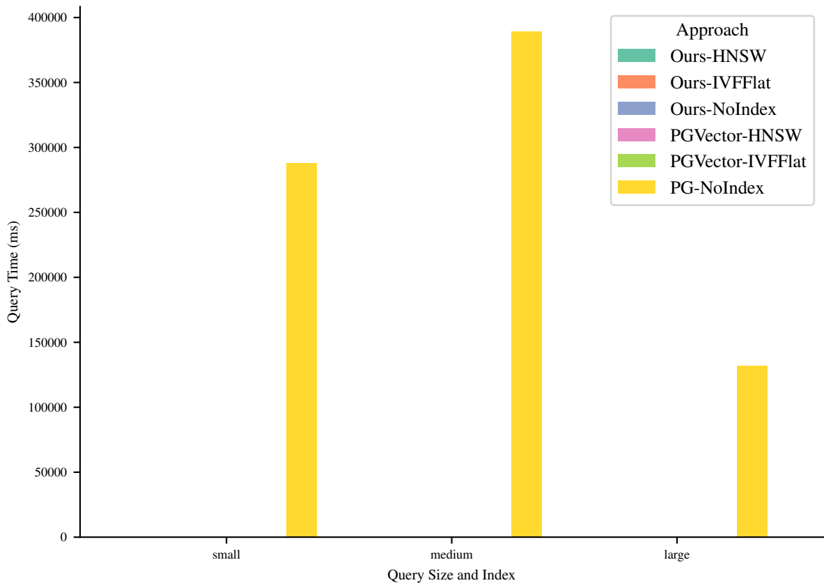
Query Time (ms) for Query 36
