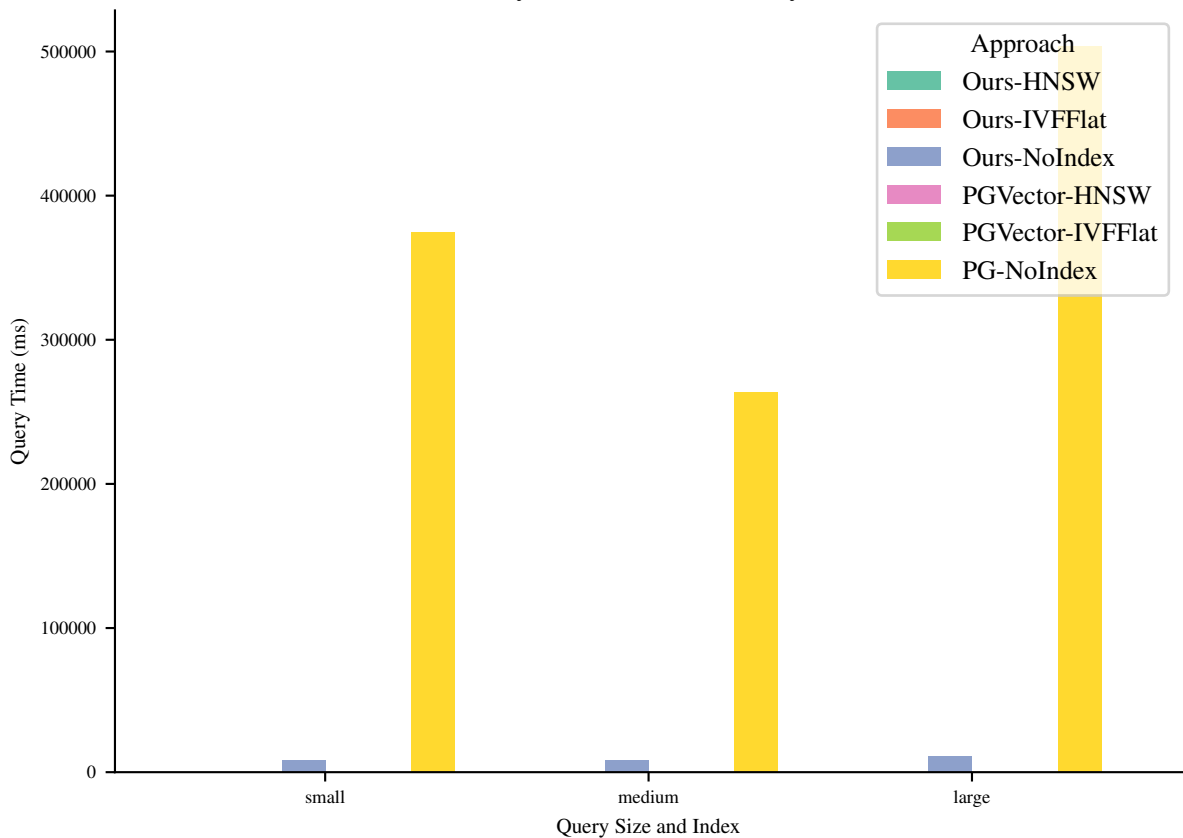
Query Time (ms) for Query 24
