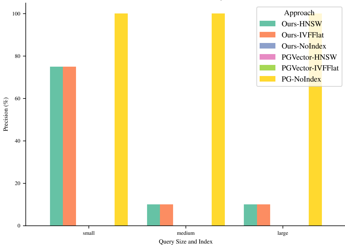
Precision (%) for Query 28
