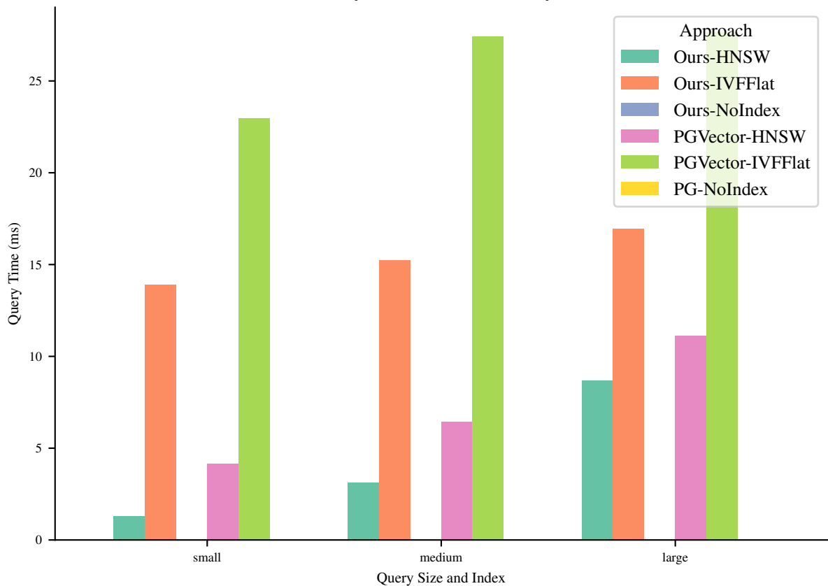
Query Time (ms) for Query 7
