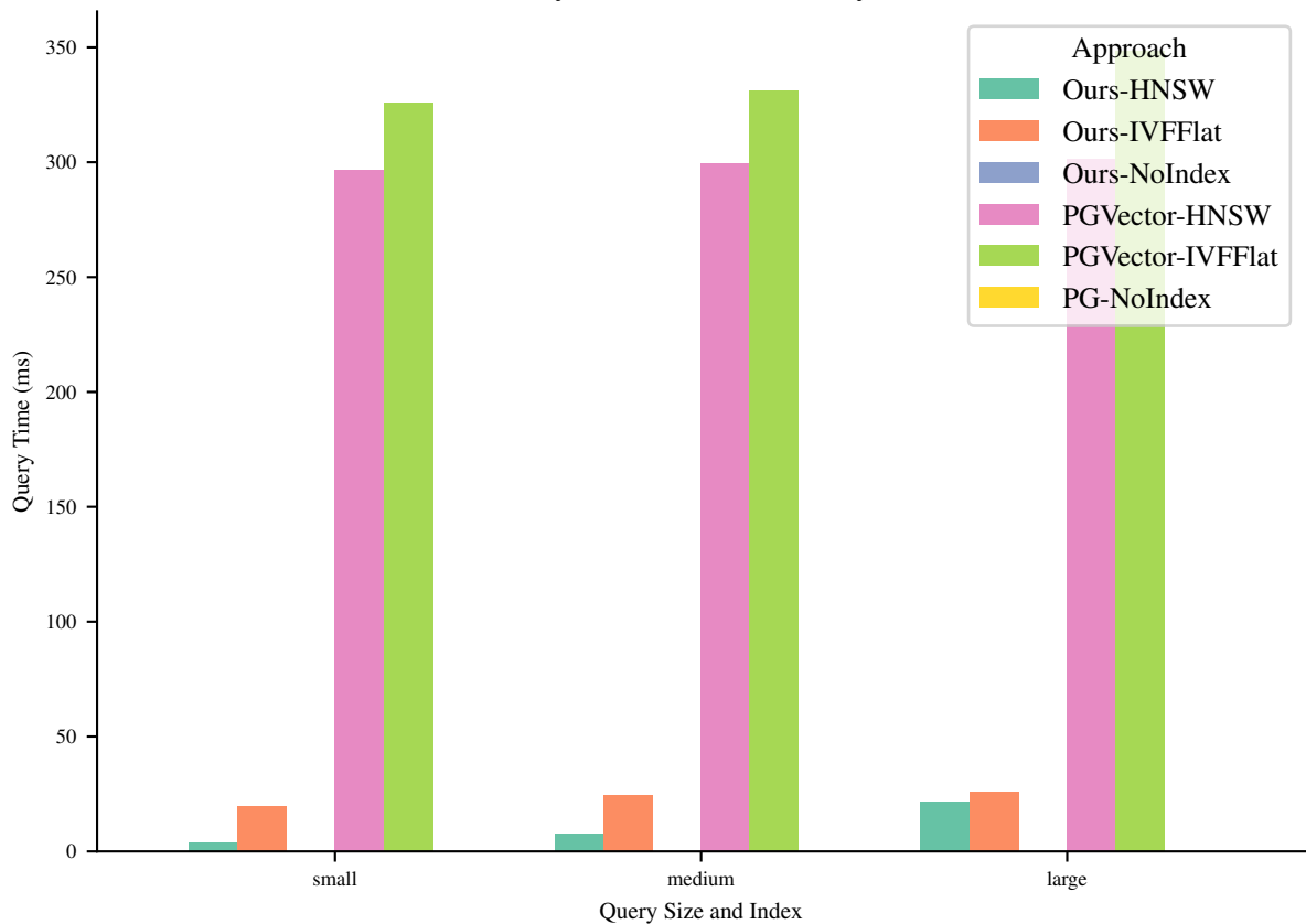
Query Time (ms) for Query 17
