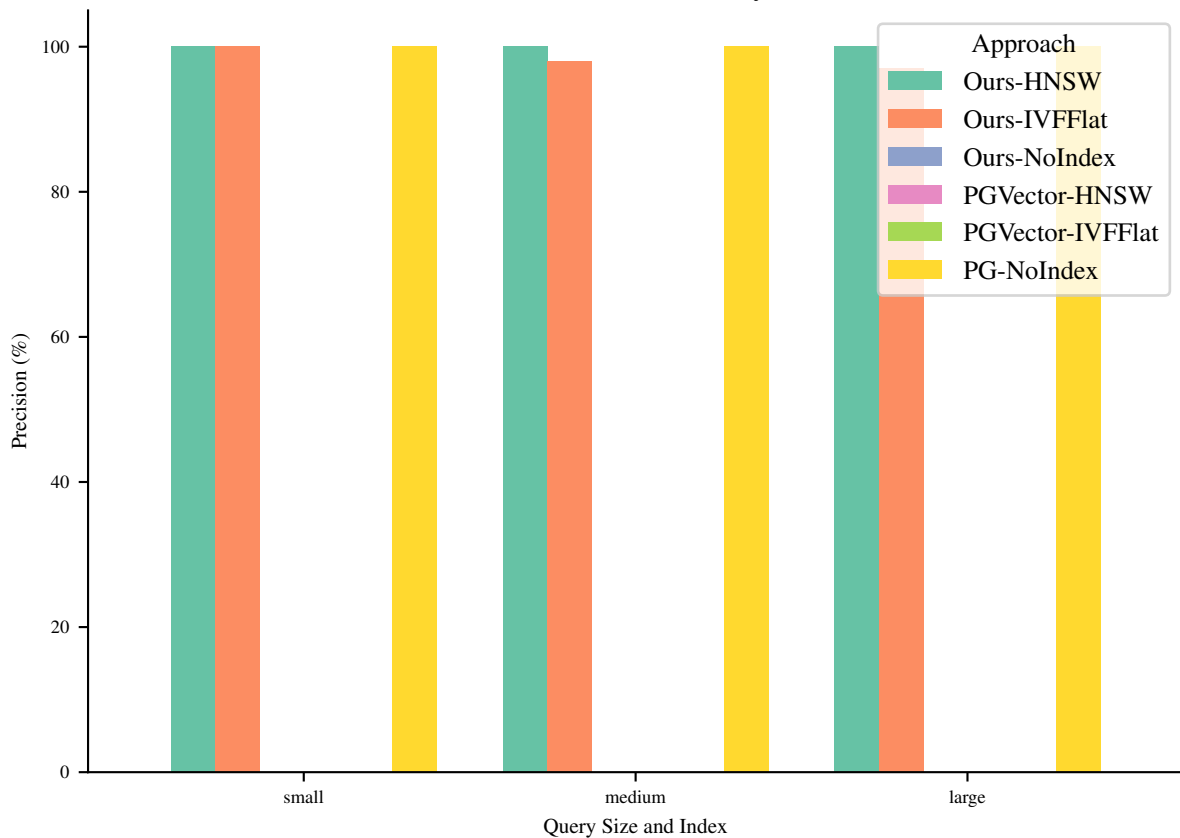
Precision (%) for Query 36
