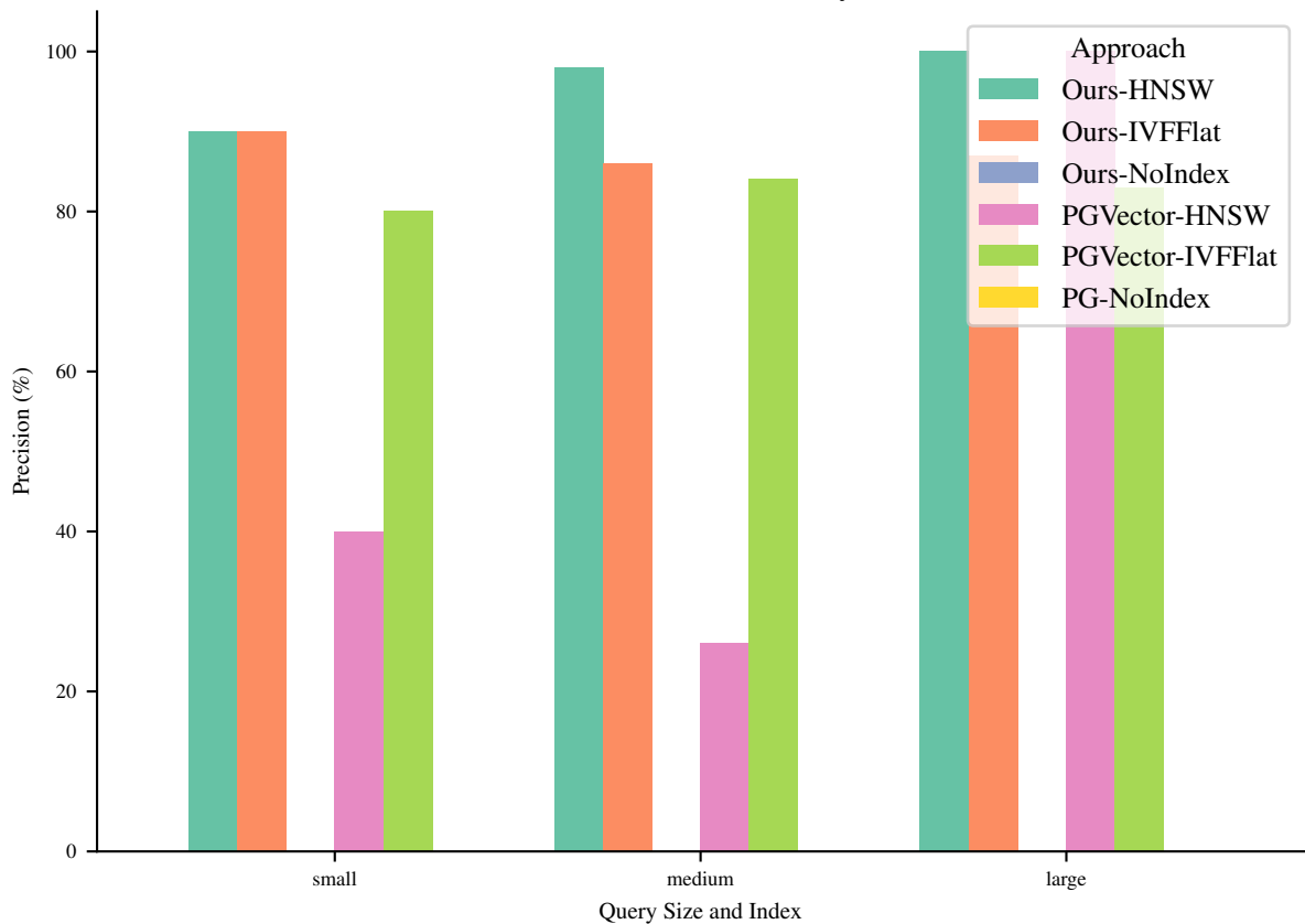
Precision (%) for Query 5
