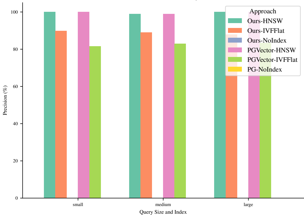
Precision (%) for Query 2
