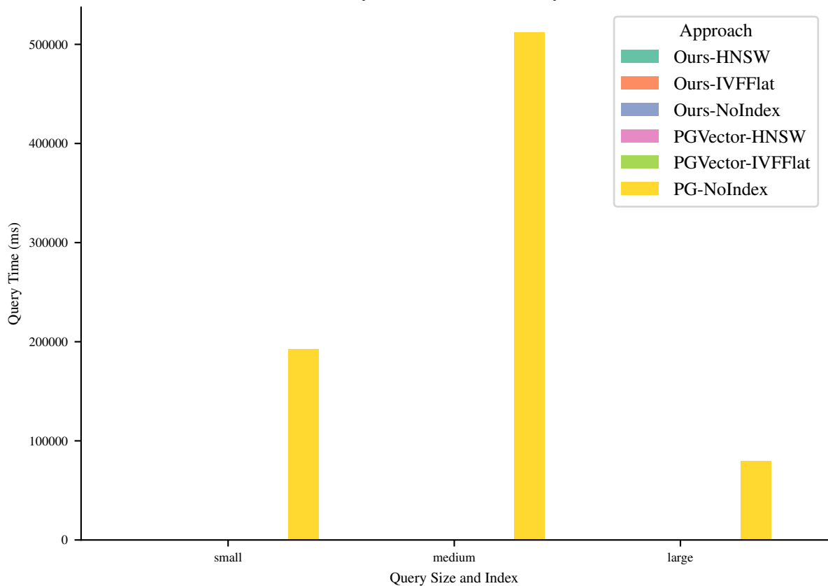
Query Time (ms) for Query 28
