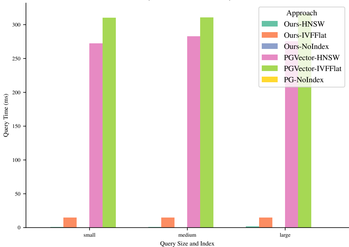
Query Time (ms) for Query 26
