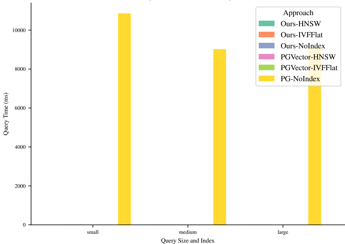
Query Time (ms) for Query 19
