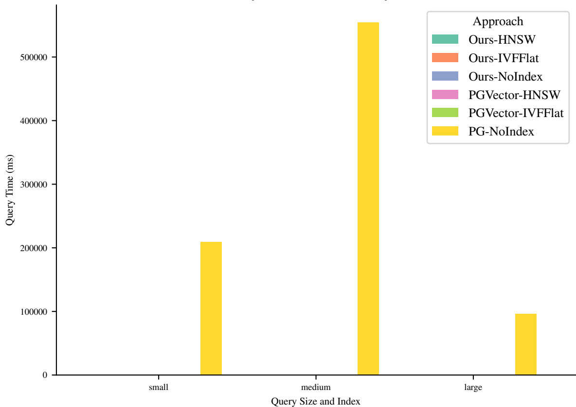
Query Time (ms) for Query 32
