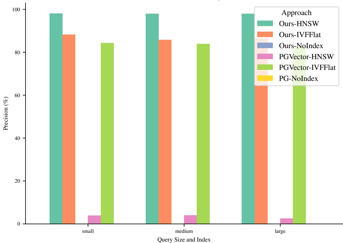
Precision (%) for Query 17
