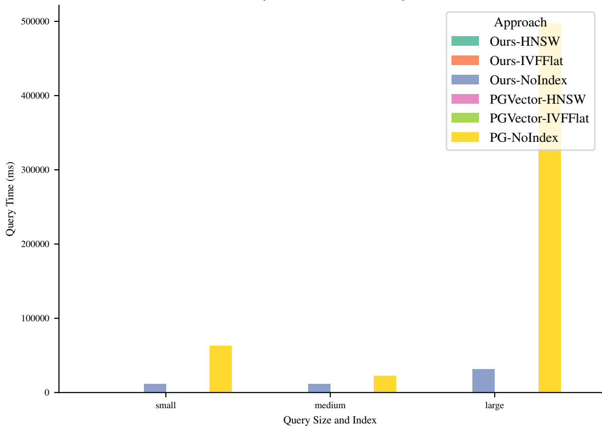
Query Time (ms) for Query 25
