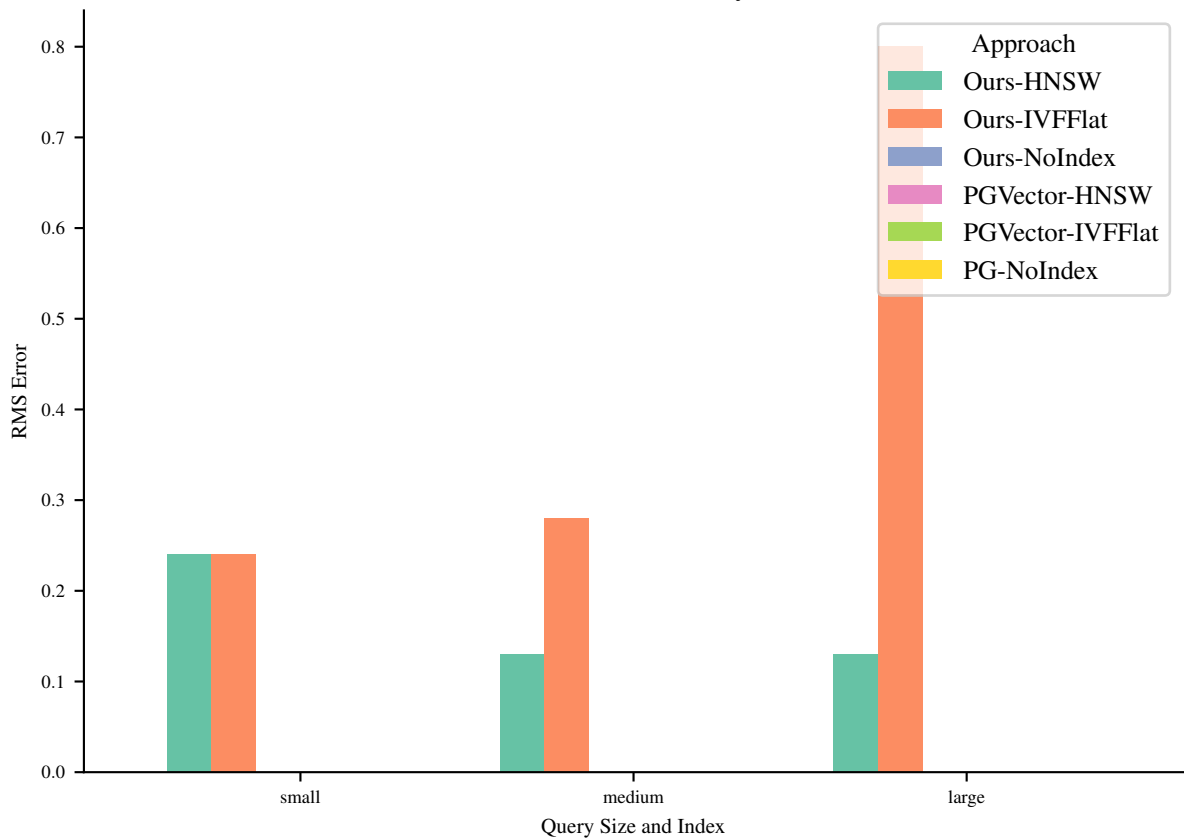
RMS Error for Query 12
