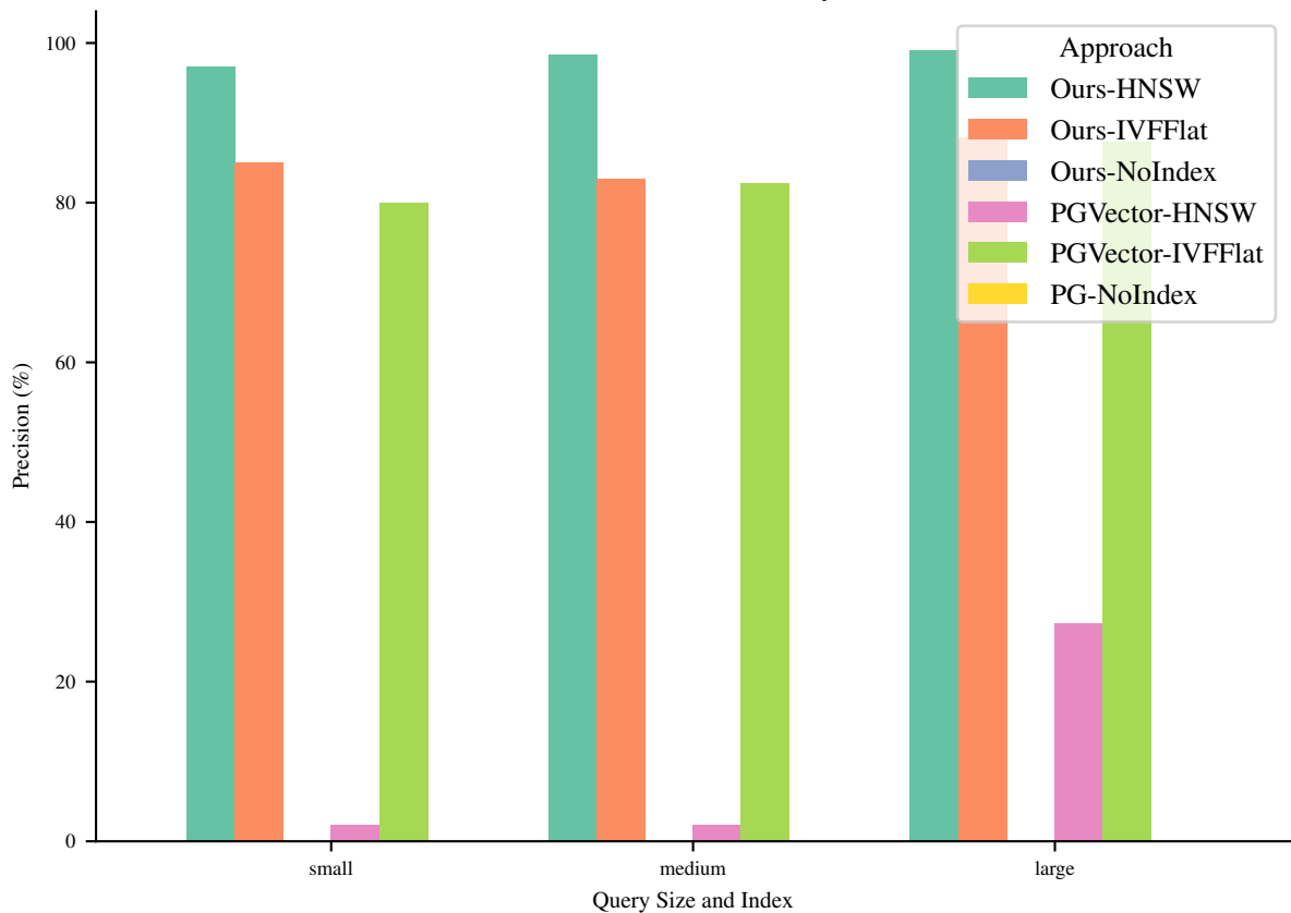
Precision (%) for Query 27
