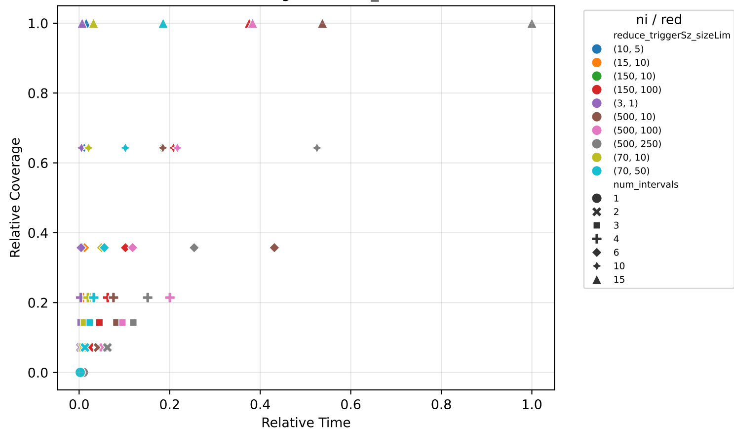
Time vs Coverage (all num_intervals)
