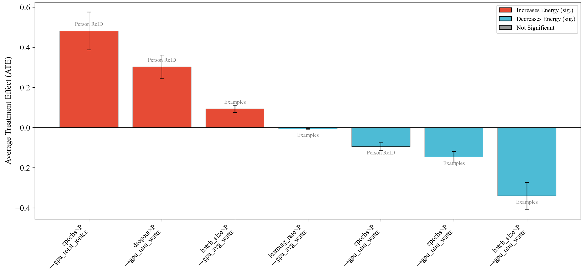
RQ1b: Parallelization Moderation Effects on Energy
