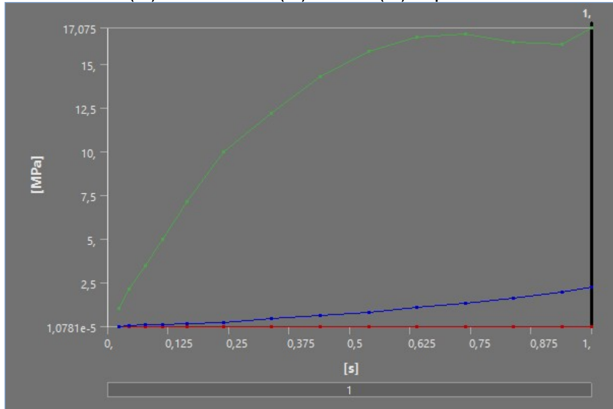
Model (B4) > Static Structural (B5) > Solution (B6) > Equivalent Stress
