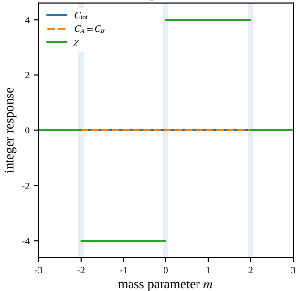
(a) One-label Chern responses
