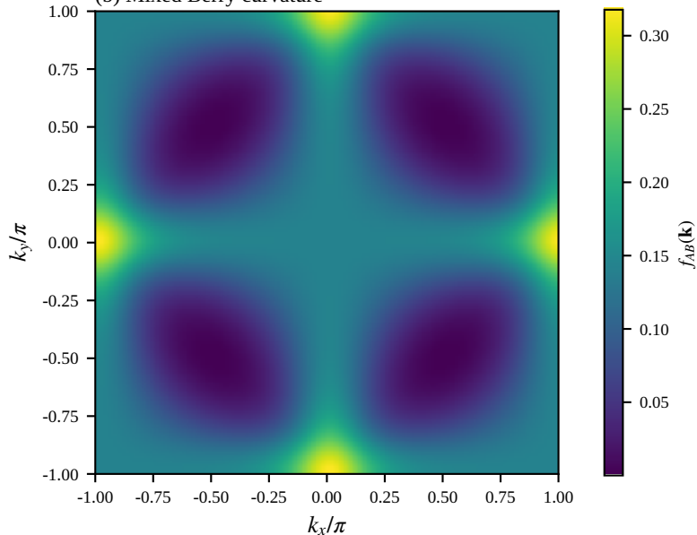
(b) Mixed Berry curvature
