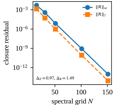
(f) Numerical residual
