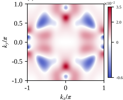
(e) Gauss-Codazzi term
