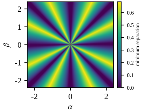
(a) Projected-label gap
