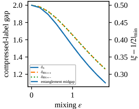
(c) Hierarchical gaps
