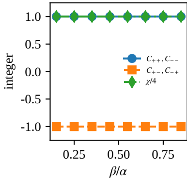
(b) Sector Chern numbers
