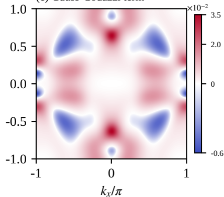
(e) Gauss-Codazzi term
