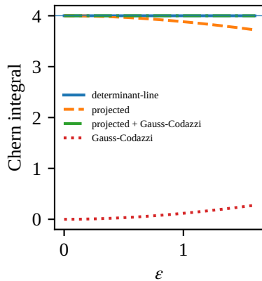
(e) Gauss-Codazzi term
