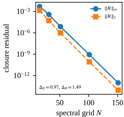
(f) Numerical residual
