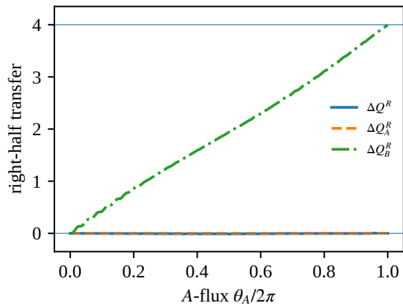
(c) Finite-time charge transfer, T = 100
