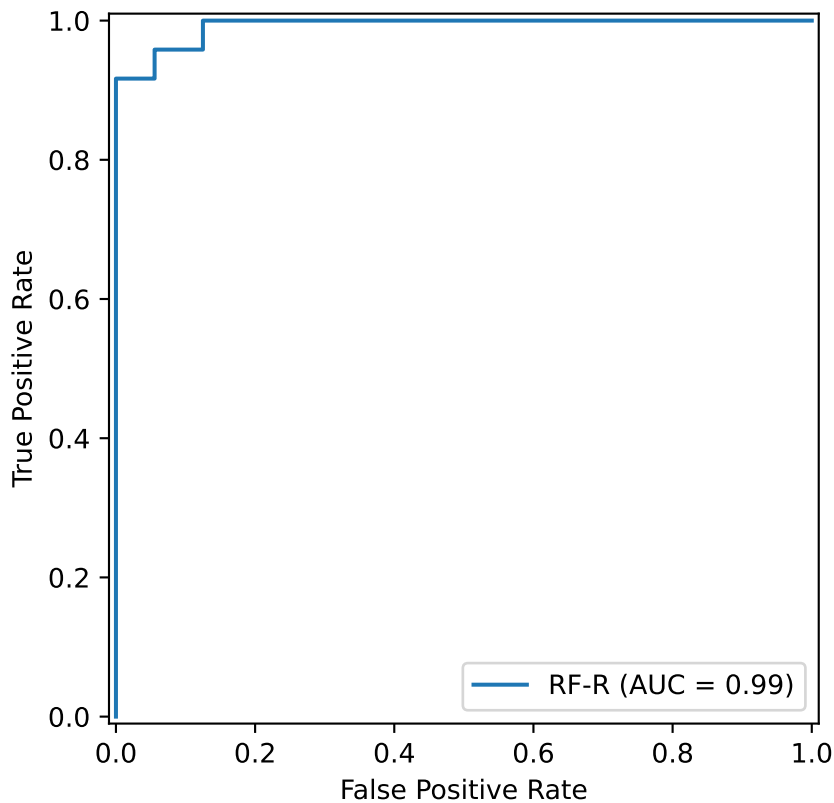
ROC - Meropenem_AB (Class R)
