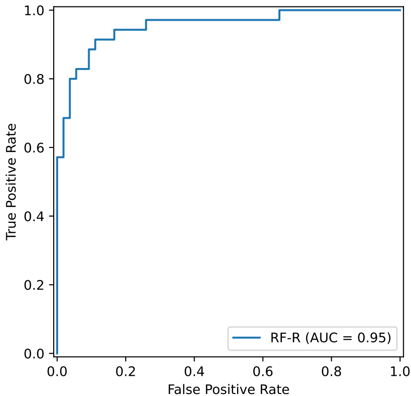
ROC - Ceftazidime_AB (Class R)
