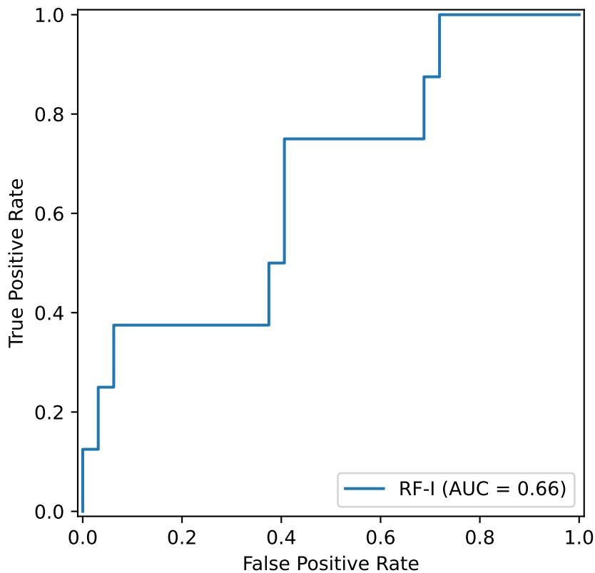
ROC - Cefepime_AB (Class I)
