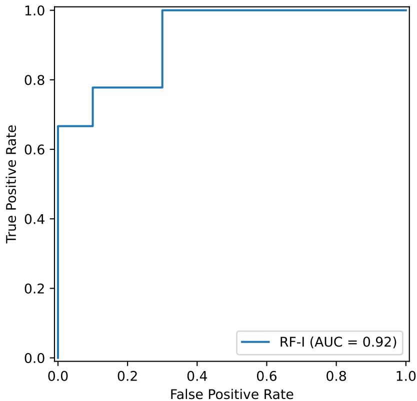
ROC - Cefuroxime_AB (Class I)
