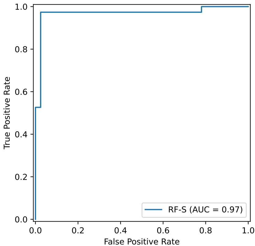
ROC - Cefotaxime_AB (Class S)
