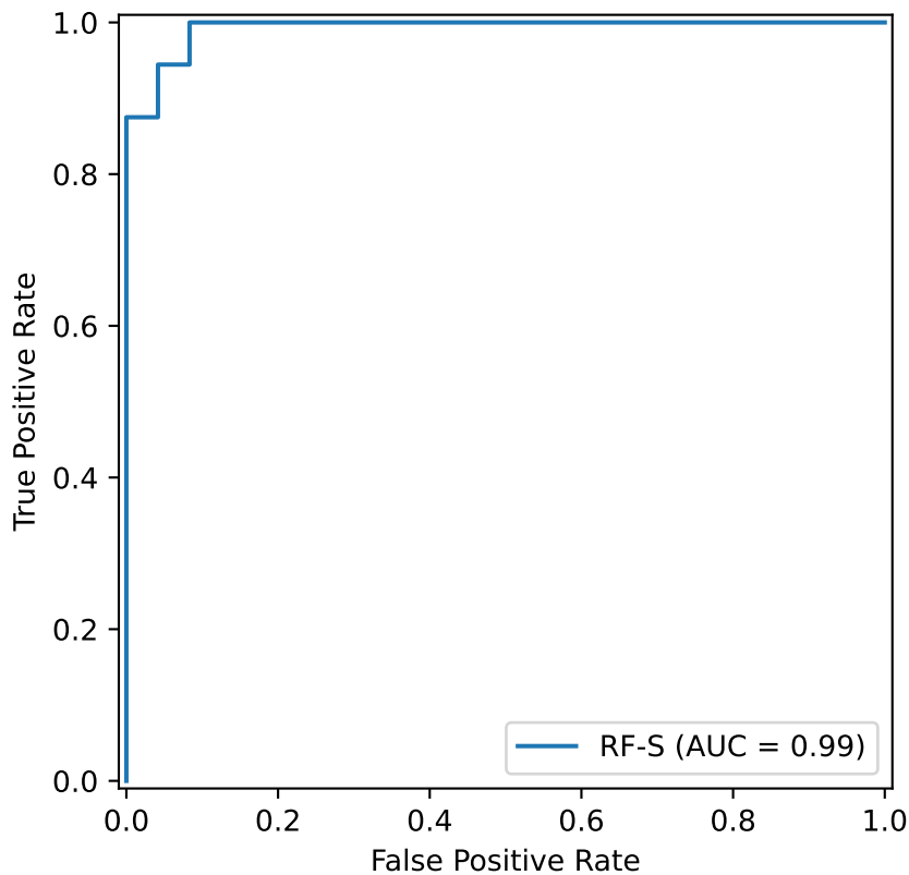
ROC - Meropenem_AB (Class S)
