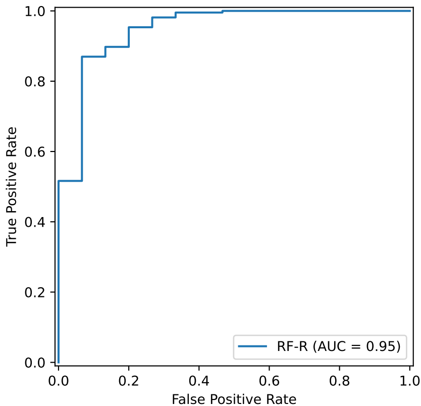
ROC - Ampicillin_AB (Class R)
