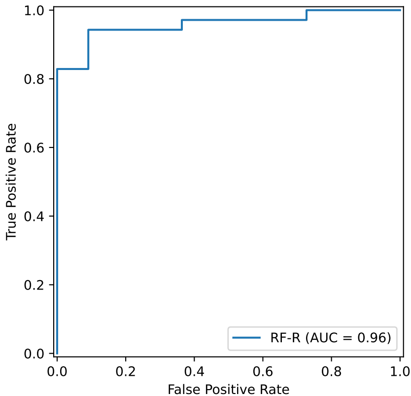
ROC - Trimethoprim_AB (Class R)
