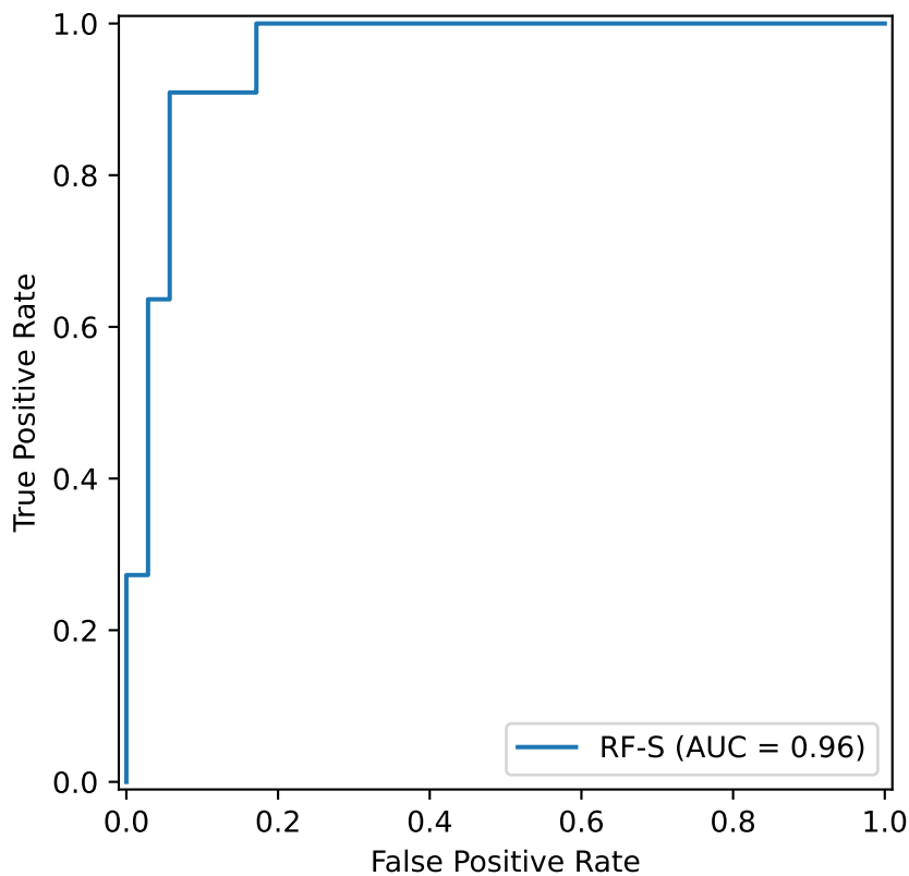
ROC - Trimethoprim_AB (Class S)
