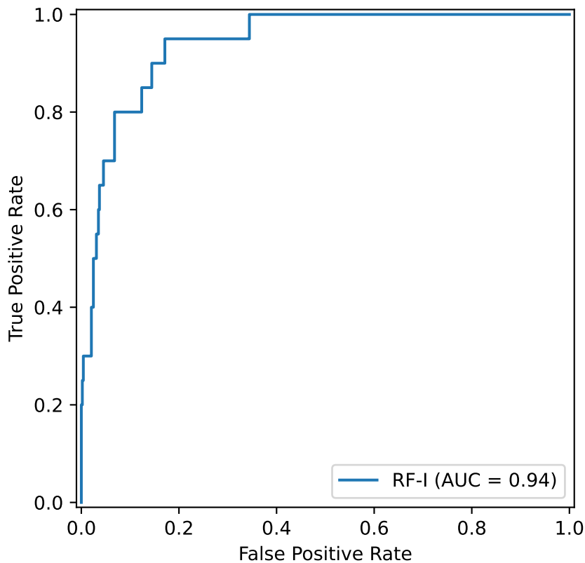
ROC - Ciprofloxacin_AB (Class I)
