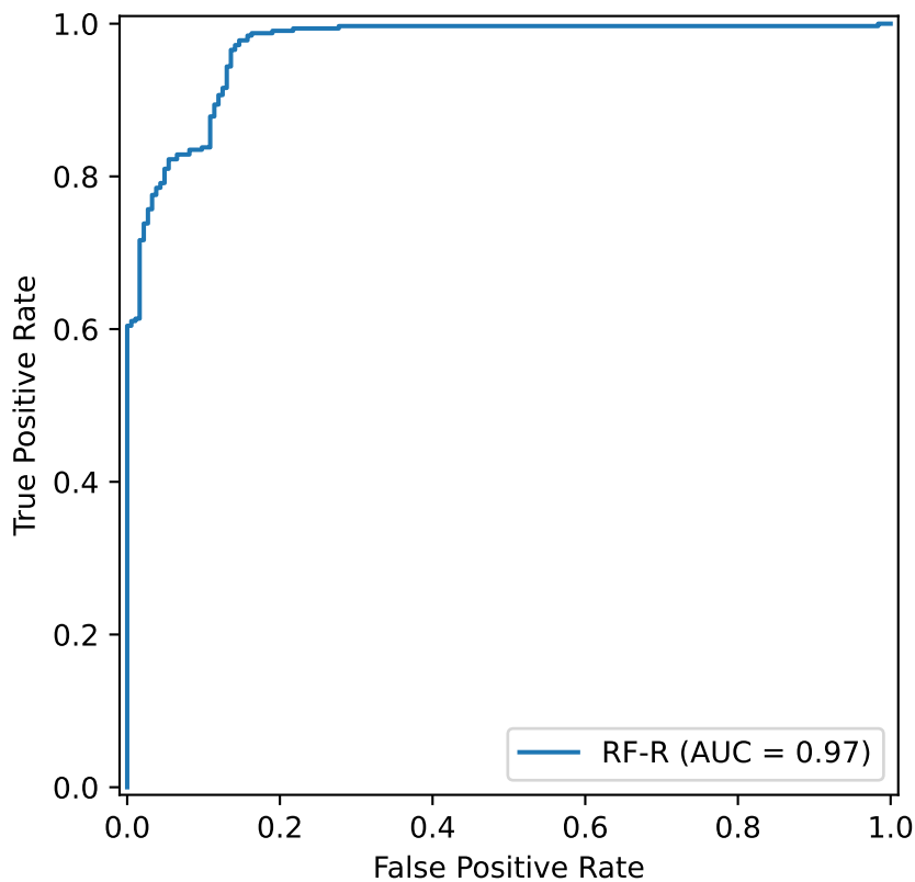
ROC - Ciprofloxacin_AB (Class R)
