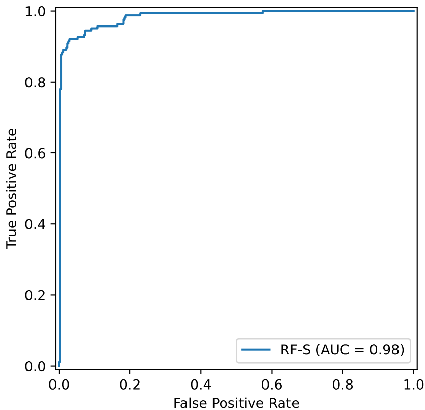
ROC - Ciprofloxacin_AB (Class S)
