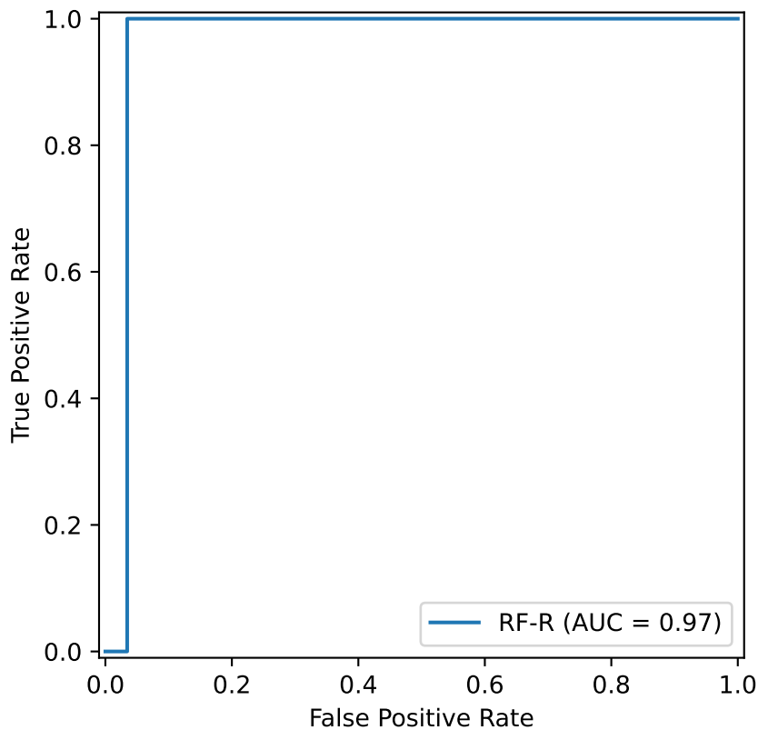
ROC - Norfloxacin_AB (Class R)
