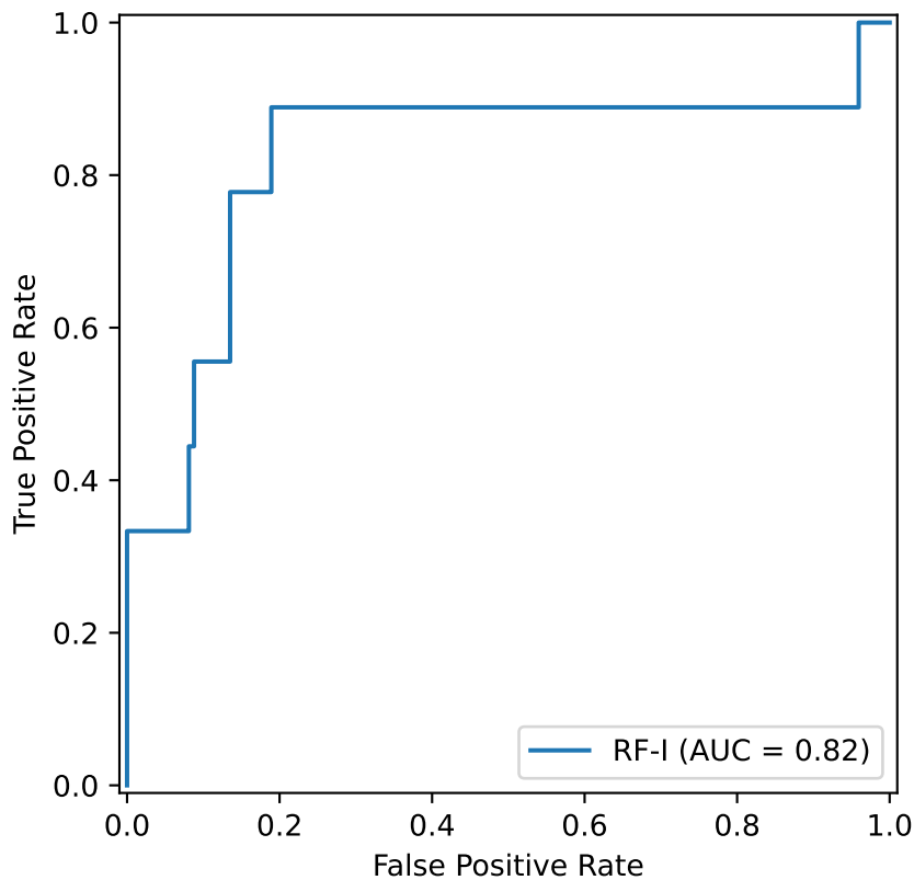
ROC - Aztreonam_AB (Class I)
