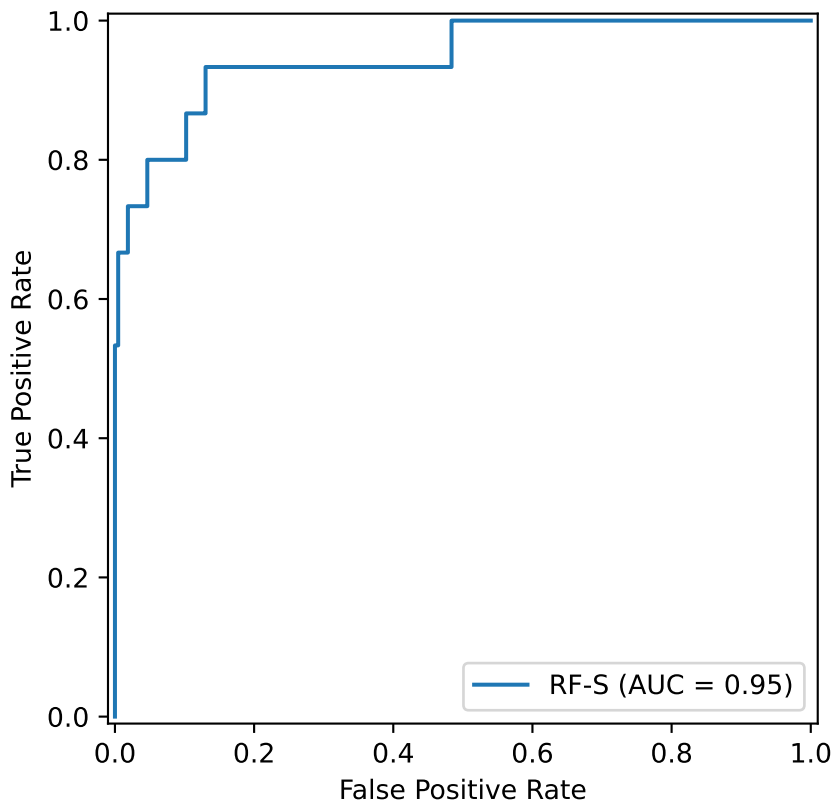
ROC - Ampicillin_AB (Class S)
