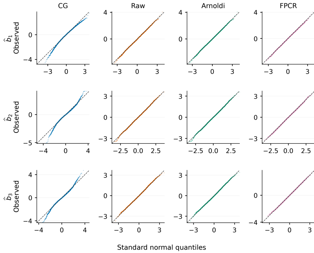
Figure F.9: Normal quantile–quantile plots for the first three estimated basis coefficients in Model 3, using the same empirical standardisation and identity reference line as in Model 1.
