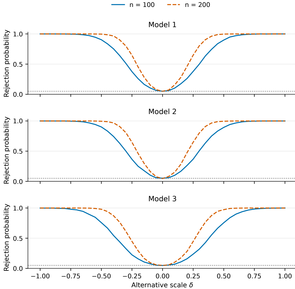
Figure H.3: Empirical power against \beta_\delta(s) = \beta(s) + \delta s . Solid and dashed curves correspond to n = 100 and n = 200 , respectively, and the dotted line marks 5%. Every point uses 5,000 alternative samples and the direct-moment statistic \mathcal{S}_n . Its empirical null critical value is calculated separately for each model and sample size. The alternatives use fixed \delta ; these are not finite- m = 70 power curves or a direct simulation of root- n local alternatives.
