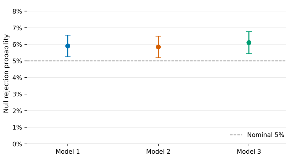
Figure I.1: Empirical null rejection probability of \mathcal{T}_{n,70} at n = 100 , using the oracle weighted chi-square 5% critical value. Each point is based on 5,000 finite-sample replications; vertical bars are normal-approximation intervals equal to the estimate plus or minus 1.96 binomial Monte Carlo standard errors. They condition on the realised critical values and do not include uncertainty from the 50,000 oracle draws. Since only oracle calibration was selected, the figure compares empirical size with the nominal line rather than comparing alternative feasible calibration procedures.
