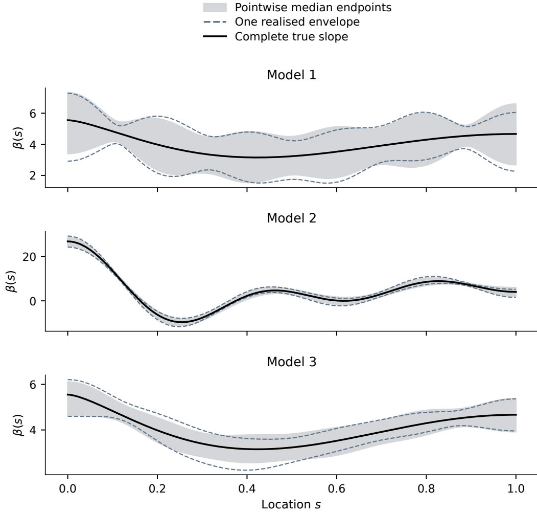
Figure H.4: Confidence-set illustration at n = 100 , using m_C = 10 , a five-dimensional analytic ellipsoid, and the oracle 5% critical value. The black curve is the complete true slope. The grey region joins the pointwise medians of the lower and upper boundaries from 5,000 separately calculated envelopes; it is not a single 95% confidence band. The dashed boundaries come from the sample whose mean envelope width is closest to the median width. All grey and dashed envelopes range only over the five-dimensional basis span. A curve can lie between the pointwise boundaries without belonging to the coefficient ellipsoid.
