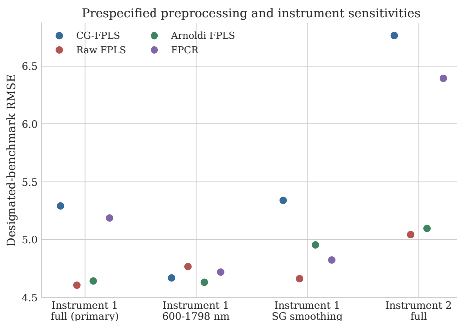
Figure K.3: RMSE across the primary analysis and three prespecified sensitivities. Points are descriptive benchmark estimates without uncertainty intervals. Horizontal comparisons change the spectral representation or instrument and do not define a post hoc replacement for the primary full-spectrum instrument-1 result.
