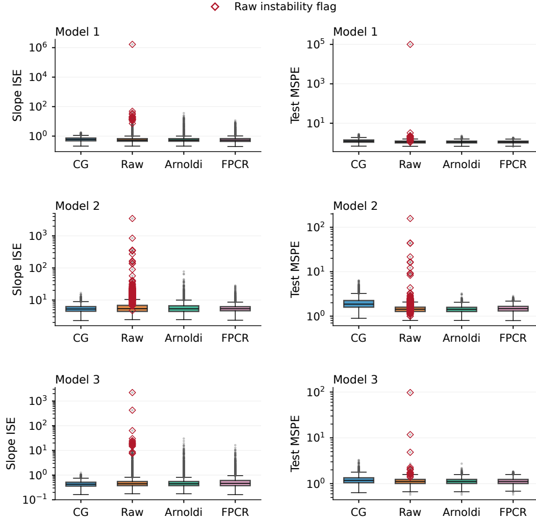
Figure E.1: Distributions of slope ISE (left column) and independent test MSPE (right column), with one row per model. The boxplots use the conventional 1.5 interquartile-range rule for their whiskers. All axes are logarithmic, and red open diamonds mark raw-FPLS fits identified as numerically unstable. The labels “CG”, “Raw”, and “Arnoldi” refer to the CG–FPLS, raw FPLS, and Arnoldi FPLS procedures defined in Appendix C. All extreme errors are retained.
