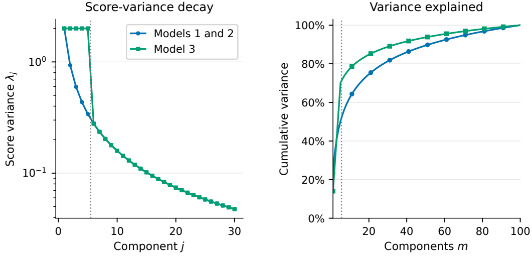
Figure D.2: Designed covariance structure. The left panel displays the first thirty score variances—the covariance eigenvalues in the continuous design—on a logarithmic scale; the right panel shows their cumulative share over all J = 100 components. The dotted vertical line separates the leading block from the common tail.
