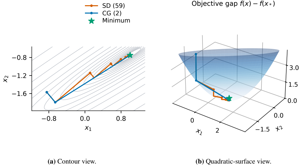
Figure C.2: Steepest descent and conjugate gradient on the same two-dimensional positive-definite quadratic with \kappa_2(A) = 50 . Steepest descent uses exact line search. The objective gap is measured relative to the common minimiser.
