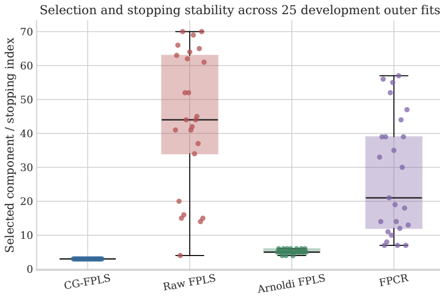
Figure J.4: Selection and stopping indices across the 25 development outer fits. Points show individual fits and boxes summarise their distributions. Raw and Arnoldi use inner cross-validation, FPCR uses GCV, and CG-FPLS uses discrepancy stopping. These counts therefore do not measure the same effective degrees of freedom.
