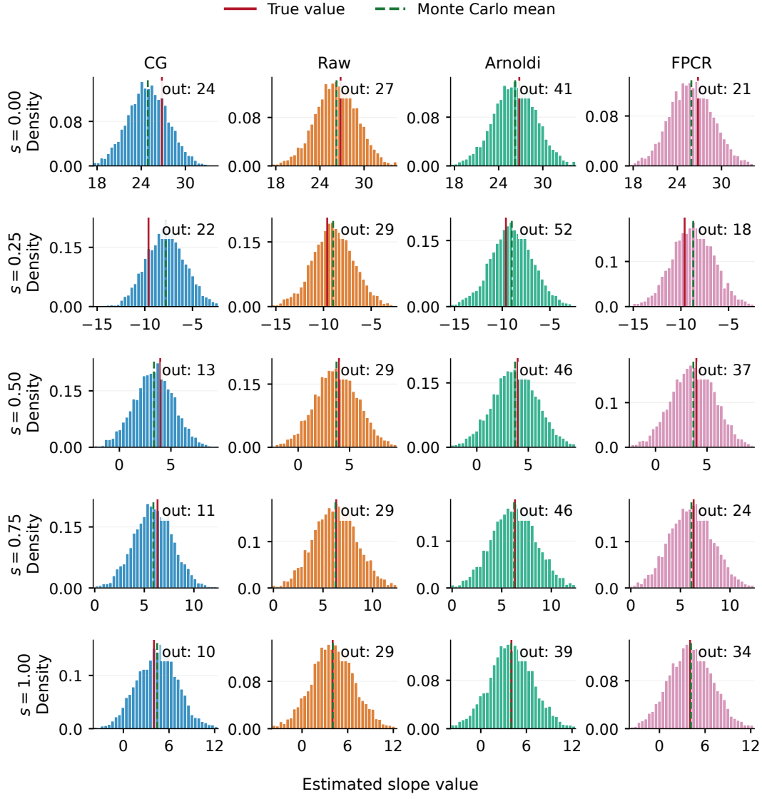
Figure F.5: Pointwise distributions of the selected slope estimator at five locations in Model 2.
