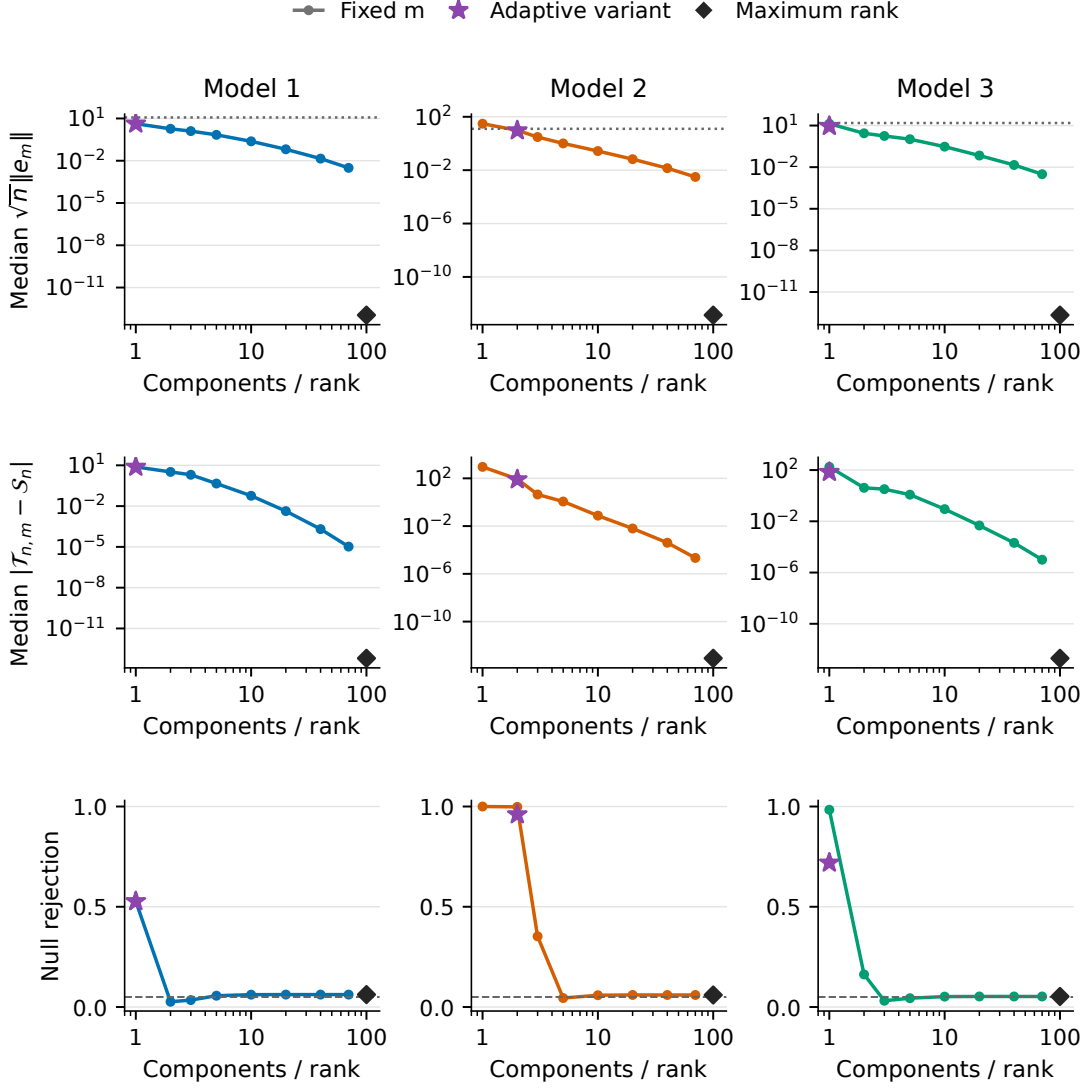
Figure H.1: Effect of the stopping index on CG-FPLS inference at n = 100 . The top row shows the median scaled moment residual \sqrt{n}\|e_m\| from (G.5). The dotted line is the median estimation-oriented stopping threshold for \sqrt{n}\|e_m\| ; it is not the vanishing residual required for inference. The middle row shows the median absolute difference between the finite- m and direct statistics, and the bottom row shows rejection under the null using the oracle 5% critical value. Circles denote fixed m , stars the adaptive variant with a 20-component pilot cap, and diamonds the maximum-rank fit. Each summary uses the 5,000 simulated samples generated for the stopping study.
