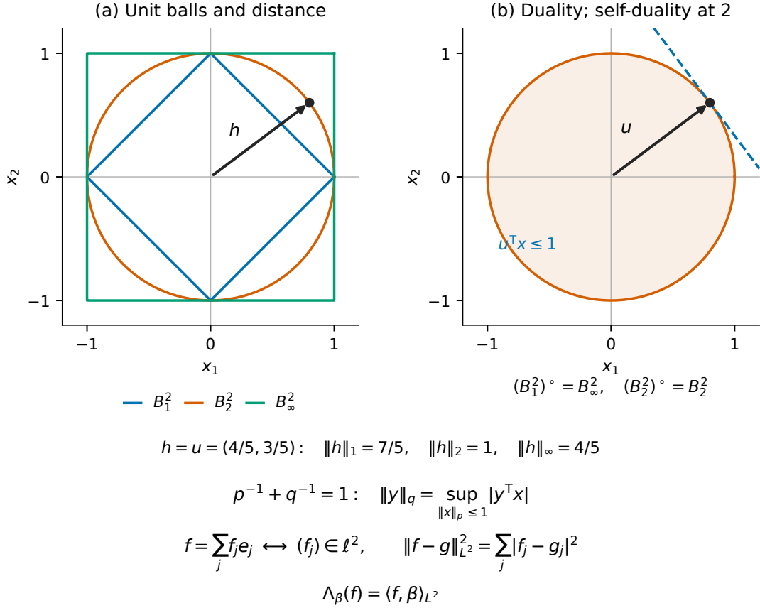
Figure A.1: Unit-ball geometry, norm-induced distance, and duality. The left panel plots B_p^2 = \{x \in \mathbb{R}^2 : \|x\|_p \leq 1\} for p = 1, 2, \infty and assigns three different lengths to the same displacement h = (4/5, 3/5) . In the right panel, q is the Hölder-conjugate exponent and (B_p^2)^\circ = B_q^2 under the standard finite-dimensional pairing. The dashed line u^T x = 1 supports the Euclidean ball at u = (4/5, 3/5) ; the same u is both the boundary point and its norming vector, illustrating (B_2^2)^\circ = B_2^2 . The lower strip records how Parseval's identity and Riesz representation transfer this self-dual coefficient geometry to L^2(\mathcal{I}) . The plotted balls are two-dimensional analogues, not depictions of infinite-dimensional sets.
