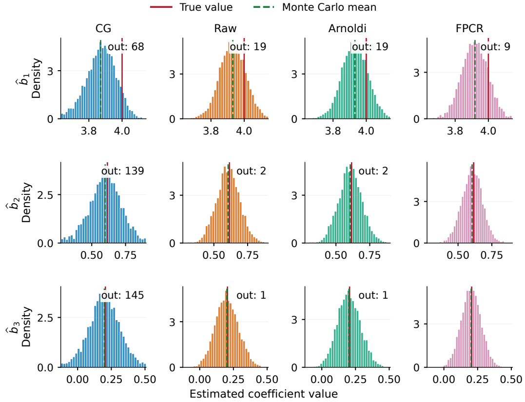
Figure F.3: Empirical distributions of the first three basis coefficients in Model 3.
