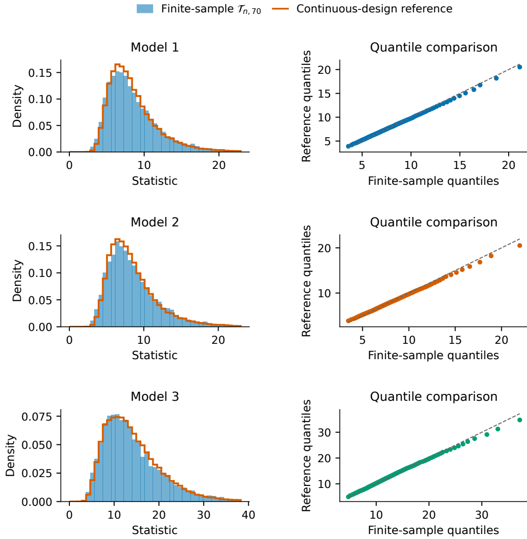
Figure H.2: Finite-sample null calibration of the late-stopped CG-FPLS test. Rows correspond to Models 1–3. The left column overlays the empirical density of \mathcal{T}_{n,70} from 5,000 samples at n = 100 with 50,000 draws from the continuous-design oracle weighted chi-square reference. The right column plots finite-sample quantiles horizontally and reference quantiles vertically against the identity line. Different density scales across models reflect the different null dispersions. Agreement is strongest in the centre; points below the line in the upper tail indicate larger finite-sample quantiles.
