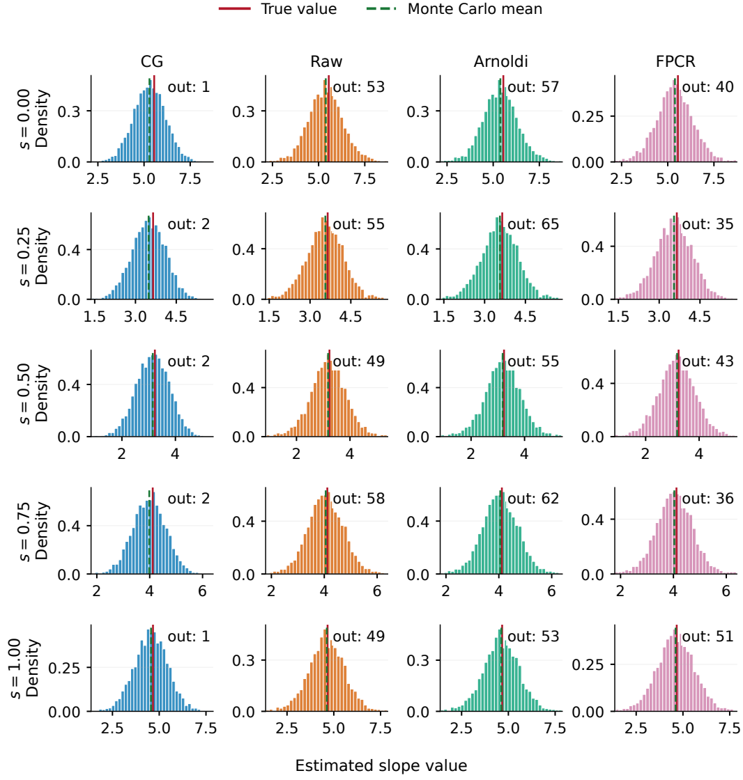
Figure F.6: Pointwise distributions of the selected slope estimator at five locations in Model 3.
