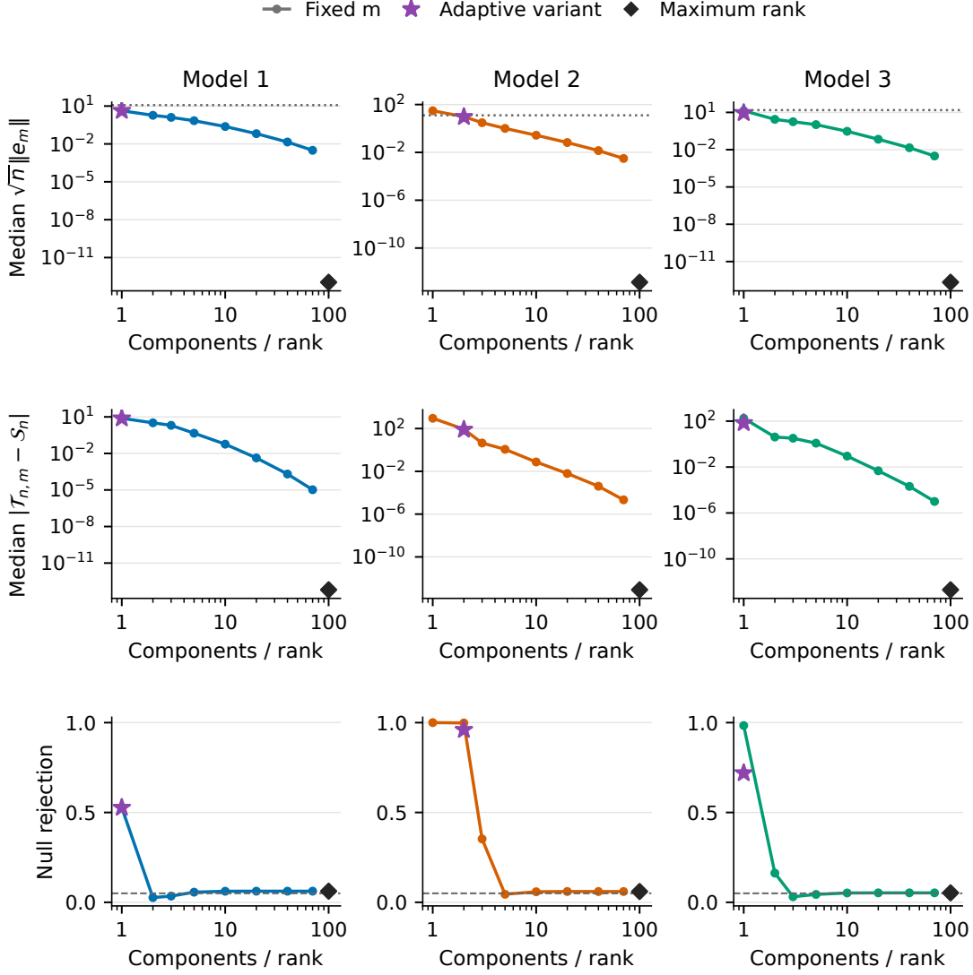
Figure 4.1: Stopping diagnostics at n = 100 , based on 5,000 samples per model in the separate stopping study. Rows show median \sqrt{n}\|e_m\| , median |\mathcal{T}_{n,m} - \mathcal{S}_n| , and oracle-calibrated null rejection at 5%. Circles denote fixed dimensions, stars the adaptive variant with the 20-component variance pilot, and diamonds the maximum-rank fit. The dotted line in the top row is the median estimation threshold, not a vanishing inferential tolerance.
