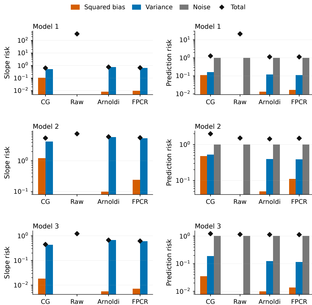
Figure E.2: Monte Carlo bias-variance decomposition over all 5,000 simulation runs. Each row is one model; slope risk is on the left and prediction risk on the right. Bars show squared bias, variance, and irreducible noise on logarithmic scales; black diamonds show total risk. The full raw-FPLS totals are included, but their components are not shown because the numerically unstable slopes are not considered reliable enough for this reconstruction.
