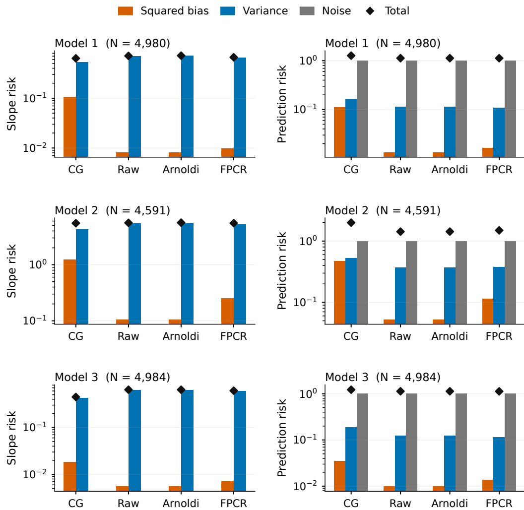
Figure E.3: Bias-variance decomposition for cases in which raw FPLS satisfies its numerical-stability rule. All four methods are evaluated on exactly the same simulation runs within each model. Each row is one model, with the number of included runs shown; slope risk is on the left and prediction risk on the right. Bar colours and black total-risk diamonds have the same meaning as in Figure E.2.
