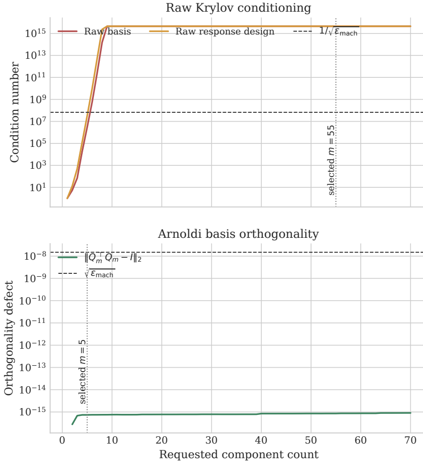
Figure K.2: Final raw and Arnoldi Krylov diagnostics. The upper panel shows raw-basis and response-design condition numbers against the fixed 1/\sqrt{\epsilon_{\text{mach}}} flag threshold. The lower panel shows Arnoldi's spectral-norm orthogonality defect; its exactly zero m = 1 value is not displayed on the logarithmic scale. Vertical markers identify the selected dimensions 55 and 5.
