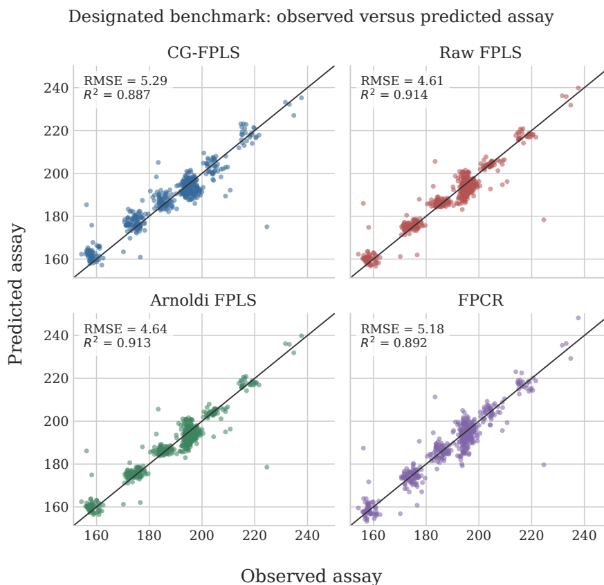
Figure 5.2: Observed and predicted assay for the 460 benchmark tablets. The diagonal denotes perfect prediction. Several large errors are shared across methods; all tablets remain in the comparison.
