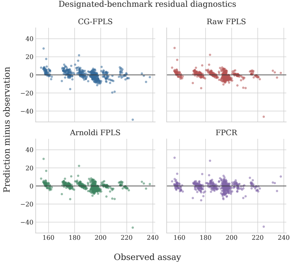
Figure K.1: Designated-benchmark residuals, defined as prediction minus observation, plotted against observed assay. All 460 tablets are retained. Shared large residuals are descriptive; the archive contains no batch or acquisition-order metadata with which to assign a physical cause.
