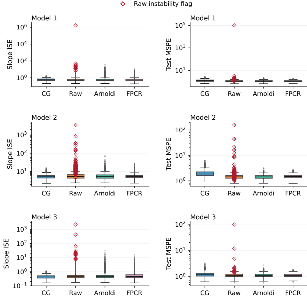
Figure 3.2: Slope ISE (left) and independent test MSPE (right), with one row per model. All errors are included on logarithmic axes. Red open diamonds identify flagged raw-FPLS fits; whiskers use the conventional 1.5 interquartile-range rule. CG, Raw, and Arnoldi denote the corresponding procedures in Chapter 2.
