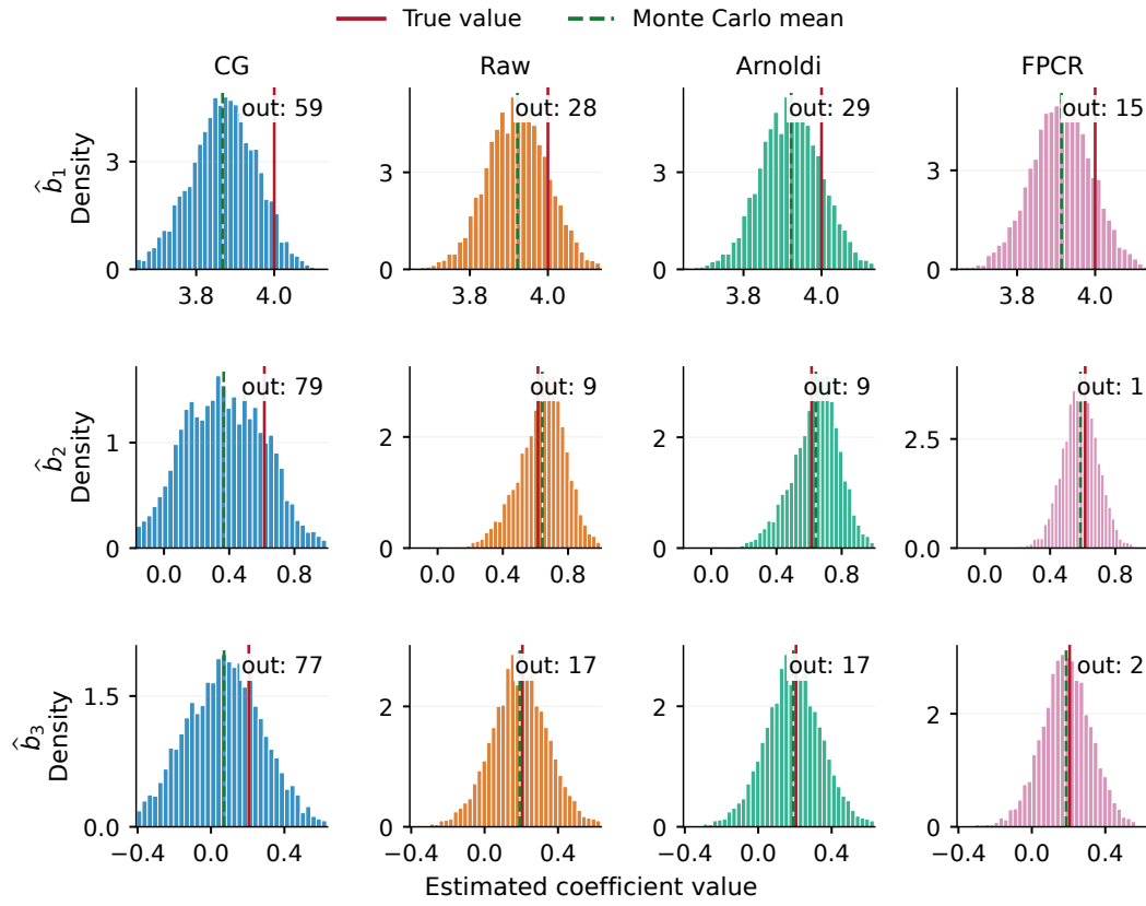
Figure F.1: Empirical distributions of the first three basis coefficients in Model 1. Solid vertical lines mark the true coefficients and dashed lines mark Monte Carlo means.
