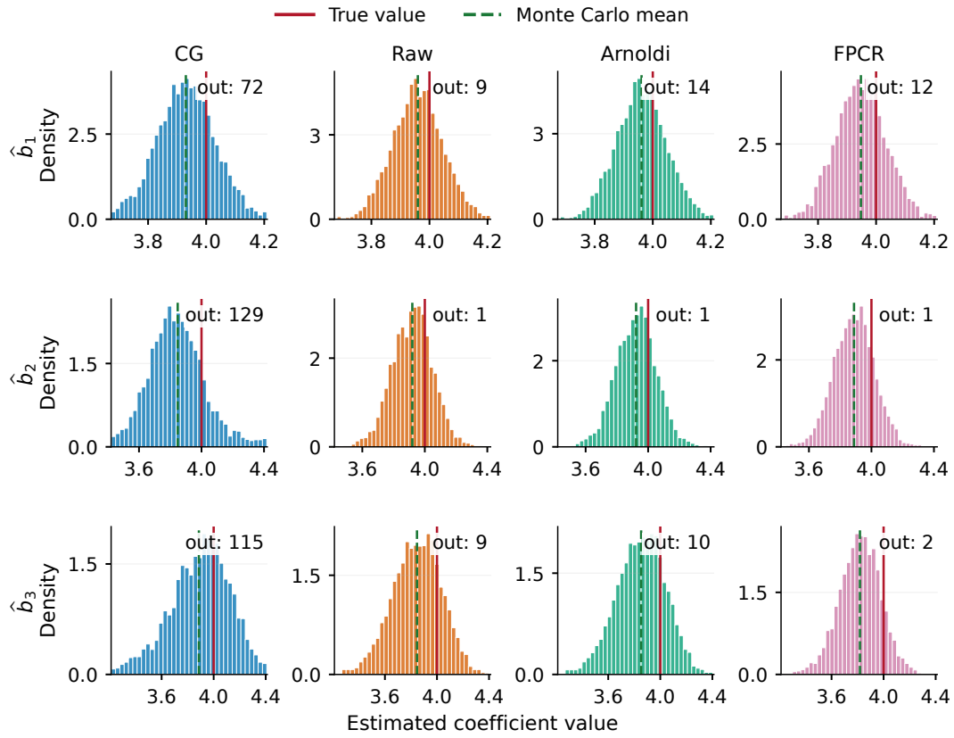
Figure F.2: Empirical distributions of the first three basis coefficients in Model 2.
