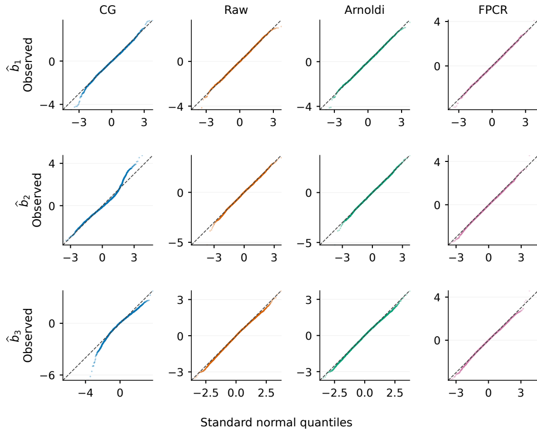
Figure F.8: Normal quantile–quantile plots for the first three estimated basis coefficients in Model 2, using the same empirical standardisation and identity reference line as in Model 1.
