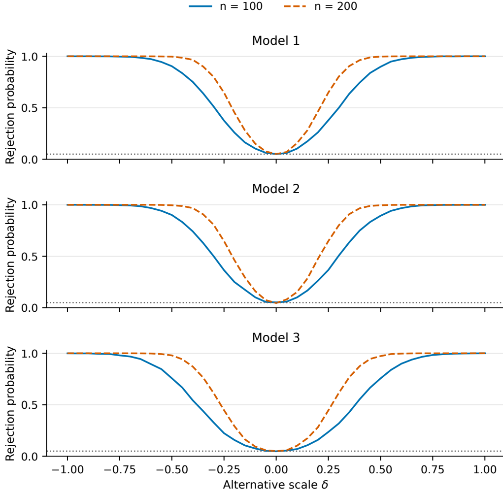
Figure 4.2: Power against \beta_\delta(s) = \beta(s) + \delta s using \mathcal{S}_n and empirical-null calibration. Solid curves use n = 100 , dashed curves n = 200 ; the dotted line marks 5%. Each point uses 5,000 separately generated alternative samples.
