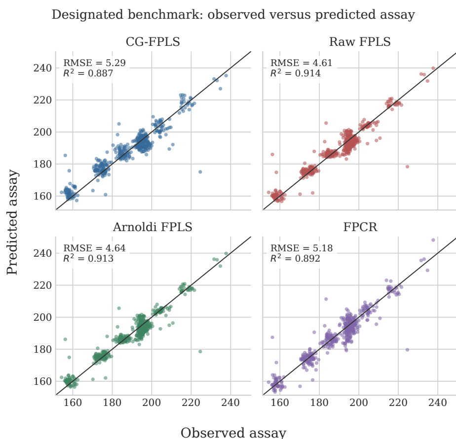
Figure J.2: Observed and predicted assay on the designated benchmark. The diagonal is the one-to-one line. The four methods capture the main linear signal and share several difficult tablets near the extremes of the assay range.
