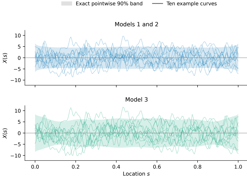
Figure D.4: Representative functional predictors and their exact pointwise 90% bands: Models 1 and 2 above, Model 3 below. The shared score draws make the spectrum change visually comparable; the actual Monte Carlo models use independent random-number streams.
