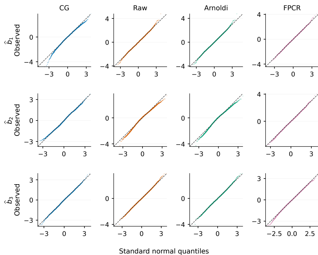
Figure F.7: Normal quantile–quantile plots for the first three estimated basis coefficients in Model 1. Each coefficient sample is standardised by its empirical mean and standard deviation; the dashed line is the 45-degree identity line.
