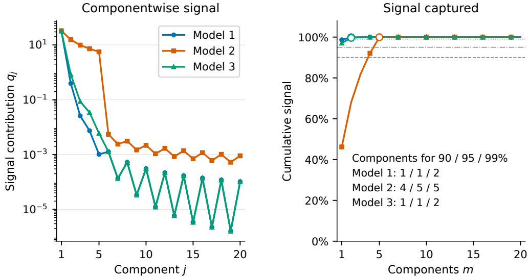
Figure D.3: Componentwise and cumulative predictive-signal allocation, calculated as q_j = \lambda_j \langle \beta, \phi_j \rangle_T^2 under the exact discrete design. Open markers denote the first component count exceeding 99% of total signal.
