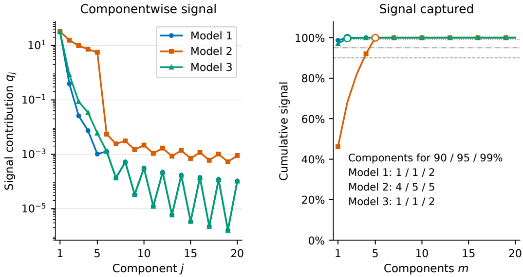
Figure 3.1: Contribution q_j = \lambda_j \langle \beta, \phi_j \rangle_T^2 of each generating direction to response signal, and its cumulative share. Calculations use all 100 directions under the endpoint-average inner product; the first twenty are displayed. Open markers identify the first component count exceeding 99% of total signal.
