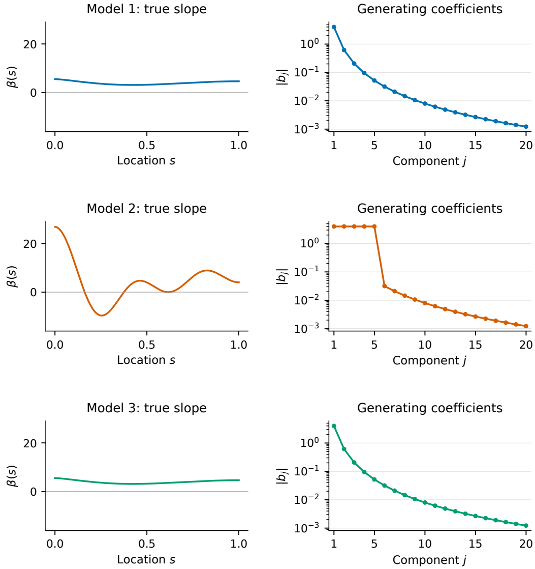
Figure D.1: True slope functions and coefficient magnitudes in the three Monte Carlo models. The curves use J = 100 functions and are evaluated on the T = 200 grid. Only the first twenty coefficients are shown in the right-hand panels; all one hundred enter the data-generating process. Rows correspond to Models 1–3, with the slope functions on the left.
