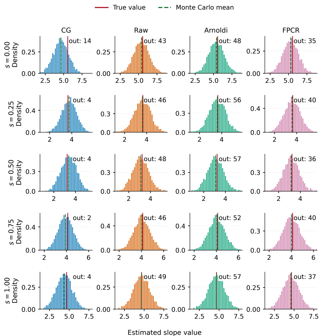
Figure F.4: Pointwise distributions of the selected slope estimator at five locations in Model 1.
