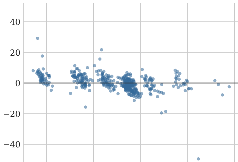
Arnoldi FPLS
