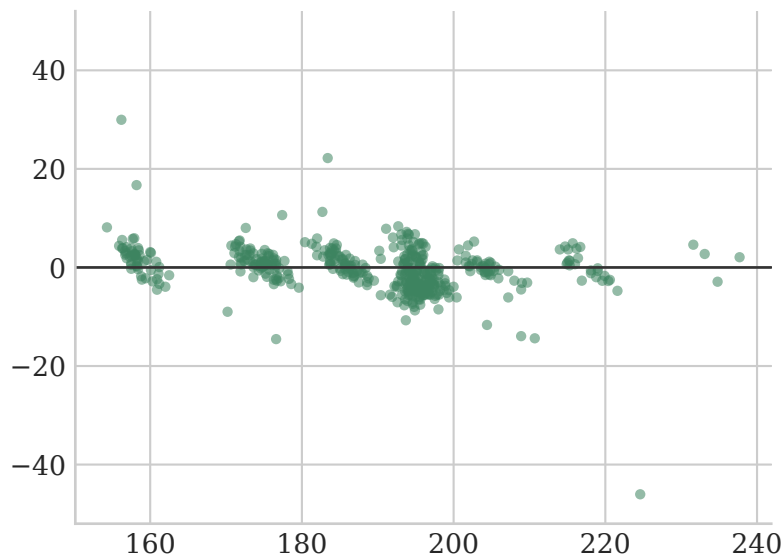
Arnoldi FPLS
