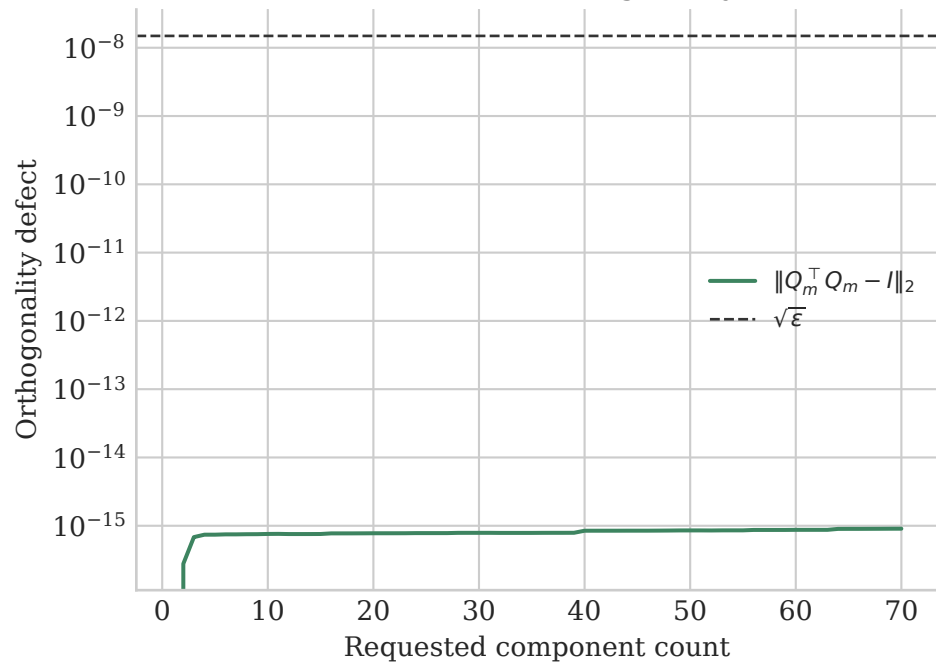
Arnoldi basis orthogonality
