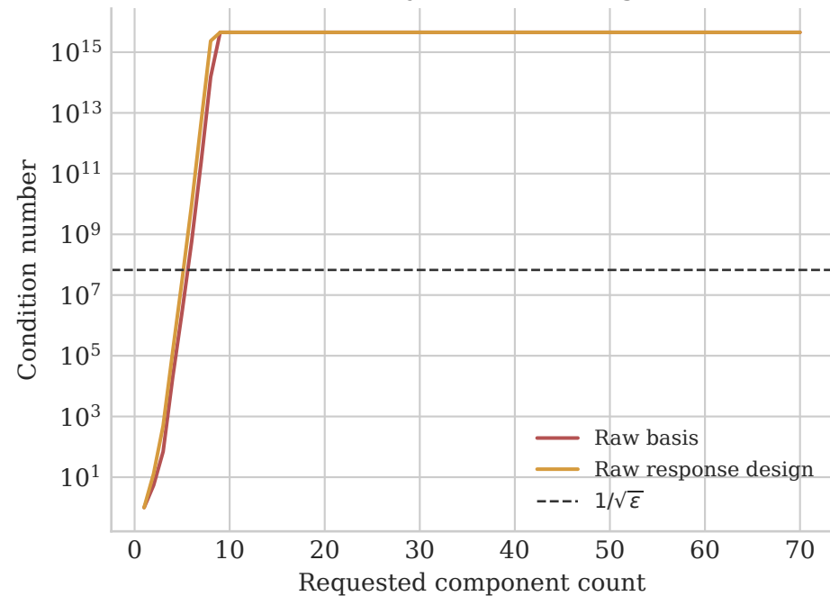
Raw Krylov conditioning
