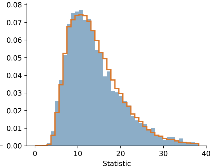
Model 3
