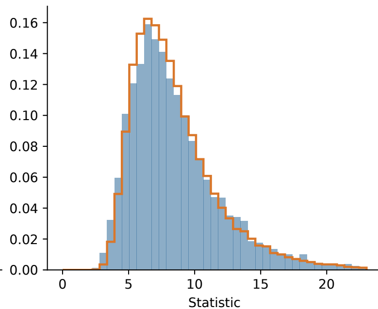
Model 2
