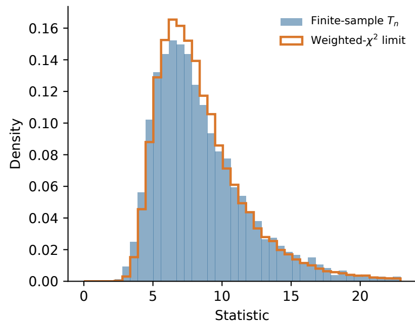
Model 1
