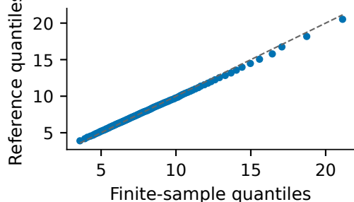
Quantile comparison
