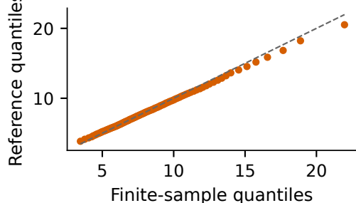
Quantile comparison
