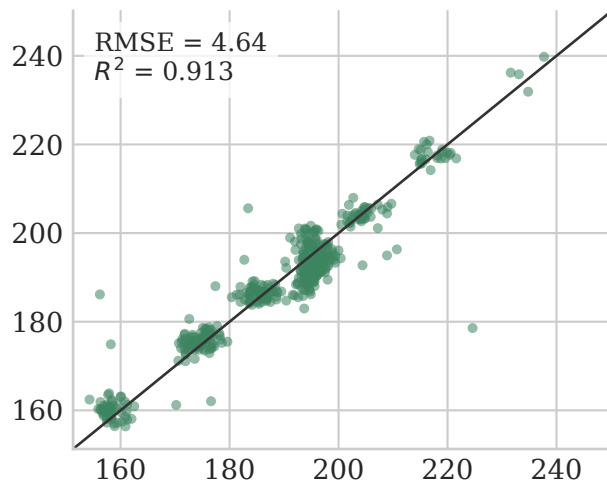
Arnoldi FPLS
