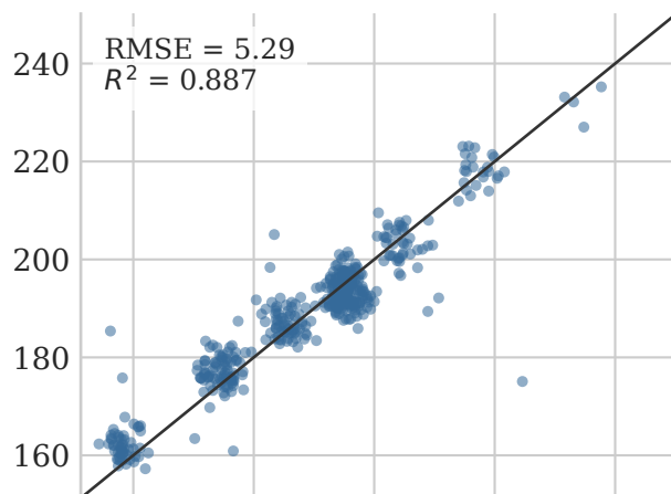
Arnoldi FPLS
